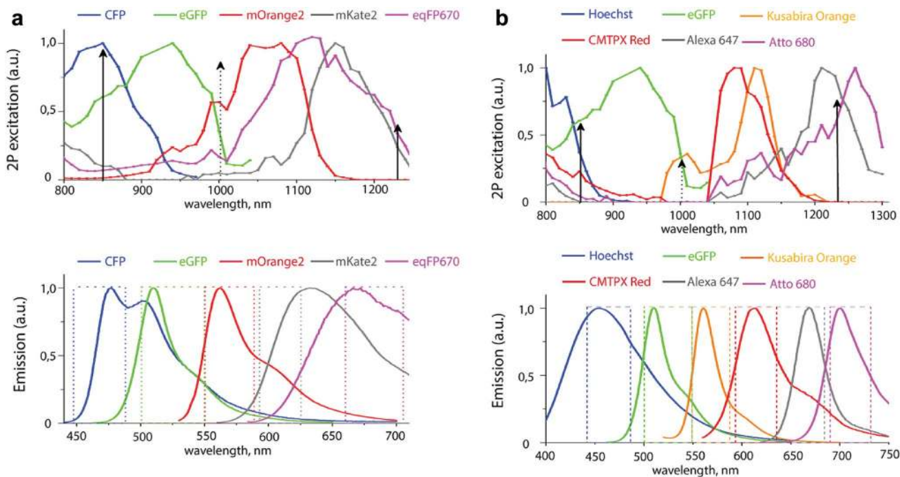
Fig. 3 Wavelength-mixing optimal combination of two sets of fluorophores. Two-photon excitation and emission spectra of two sets of fluorophores that can be efficiently excited by wavelength mixing with \lambda_1=850 nm and \lambda_2=1230 nm (full arrows), resulting in \lambda_v=1005 nm (dashed arrow). A CFP, eGFP, mOrange2,
