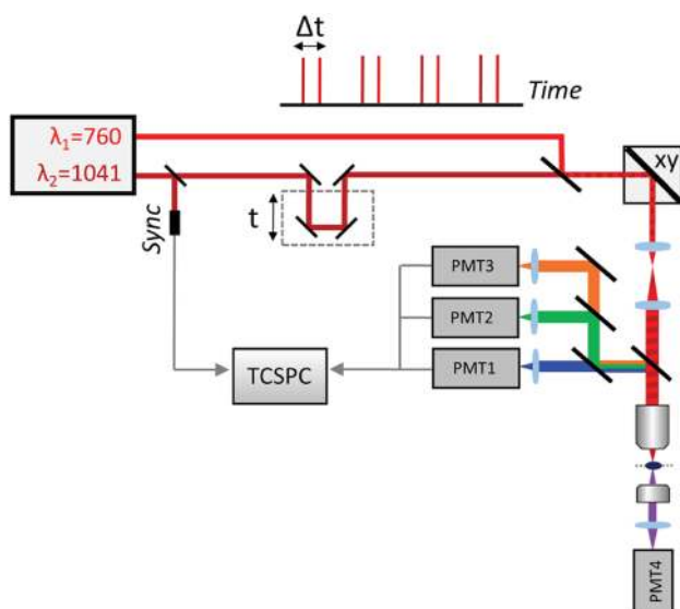
Fig. 2 Wavelength-mixing-fluorescence lifetime imaging of endogenous fluorophores. When the excitation beams \lambda_1=760 nm and \lambda_2=1041 nm are synchronized ( \Delta t=0 ), a third virtual wavelength for two-photon excitation \lambda_v=879 nm is created by wavelength mixing. A time-correlated single photon counting system (TCSPC) is used to perform FLIM. Originally published in Scientific reports (Stringari et al. 2017) under a Creative Commons Attribution 4.0 International License ( http://creativecommons.org/licenses/by/4.0/ )
