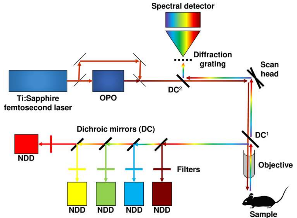
Fig. 1 Optical setup for multi-color two-photon microscopy. DC dichroic mirror, NDD non-descanned detector, OPO optical parametric oscillator. 1 Dichroic mirror used to collect fluorescent photons on five non-descanned detectors. Excitatory infrared photons pass through the mirror, whereas fluorescence photons are reflected. This mirror must be removed to collect photons in descanned mode. 2 Dichroic mirror used to collect fluorescent photons on a spectral chip in descanned mode. Modified from (Ricard and Debarbieux 2014)
