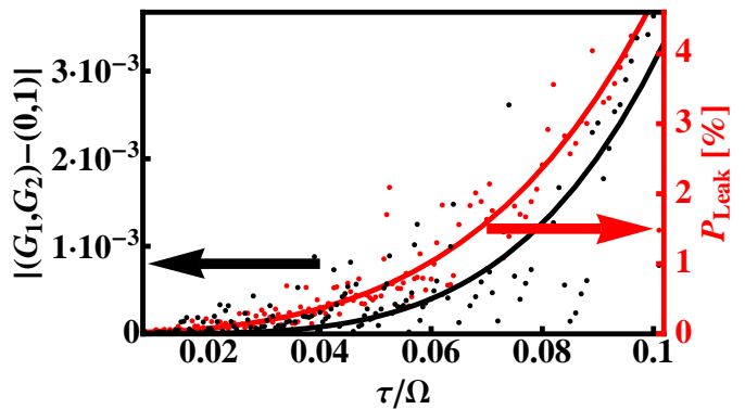
Figure 3. Numerically optimized gate sequences according to Eq. (4) for \Omega = \Omega_L = \Omega_R and \tau = \tau_i , i = 1, \dots, 4 . The deviations of the Makhlin invariants 20 from G_1 = 0 and G_2 = 1 and the leakage errors P_{\text{Leak}} are numerically minimized by adjusting the waiting times and waiting positions. P_{\text{Leak}} = |U_{\mathcal{P}\mathcal{Q}}|^2 is the transition probability from the computational subspace \mathcal{P} to the leakage subspace \mathcal{Q} . The points describe single numerical results; the solid lines are a polynomial fit. Note that small \tau/\Omega permit better gates.
