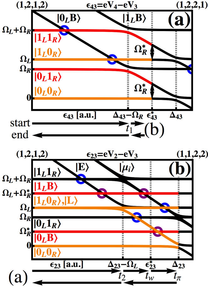
Figure 2. Energy diagram of two coupled Hqs with s_z = 1 in (1, 2, 1, 2) , (1, 2, 2, 1) , and (1, 1, 2, 2) . The red and the orange lines describe computational basis, and the black lines are leakage states. (1, 2, 1, 2) is favored without external bias. (a) shows the pulsing towards (1, 2, 2, 1) , which is modeled through \epsilon_{43} = eV_4 - eV_3 describing the potentials at QD 3 and QD 4 . The states |1_L 1_R\rangle and |1_L B\rangle as well as |0_L 1_R\rangle and |0_L B\rangle are swapped at \epsilon_{43} = \Delta_{43} - \Omega_R . Two of the four state combinations from the computational basis remain in (1, 2, 1, 2) at \epsilon_{43} = \epsilon_{43}^* . (b) shows the second step of the manipulation. \epsilon_{23} = eV_2 - eV_3 models the potentials at QD 2 and QD 3 . As a consequence, only |1_L 0_R\rangle and |0_L 0_R\rangle can be tuned to (1, 1, 2, 2) , but |1_L B\rangle and |0_L B\rangle remain in (1, 2, 2, 1) . The nontrivial part of the entangling gate is a \pi -phase evolution of |0_L 0_R\rangle at \epsilon_{23} = \Delta_{23} . |1_L 0_R\rangle is degenerate with |L\rangle and passes through a DLZC at \epsilon_{23} = \Delta_{23} - \Omega_L . Leakage from the computational subspace is prevented by the pulse cycle that involves waiting times at \epsilon_{23} = \Delta_{23} - \Omega_L and at \epsilon_{23} = \epsilon_{23}^* (see description in the text). The setup is brought back to the initial configuration in the end, by first changing \epsilon_{23} and then changing \epsilon_{43} . Perfect state crossings are marked, where transitions are forbidden from spin-selection rules (blue), or from charge-selection rules (purple). The waiting times t_1 , t_2 , t_w , and t_\pi are given in the text.
