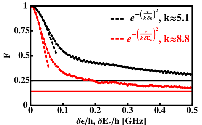
Figure 4. Fidelity analysis for the numerically optimized CPHASE gates under charge noise (black) and nuclear spin noise (red) at \Omega_L/h = \Omega_R/h = 15 GHz and \tau/h = \tau_i/h = 0.5 GHz, i = 1, \dots, 4 . The energy fluctuations \delta\epsilon between different charge configurations model charge noise. Nuclear spins cause local, low-frequency magnetic field fluctuations of the energy \delta E_z . Both noise sources can be described by a classical probability distribution with the rms \delta\epsilon (for charge noise) and \delta E_z (for nuclear spin noise). The fidelity F is extracted from 1000 gate simulations according to Eq. (4). Increasing the uncertainties suppresses F strongly till it saturates at 0.25 (for charge noise) and 9/64 (for nuclear spin noise) (see the horizontal lines). The initial decay of F is described by a Gaussian decay law (see the dotted lines).
