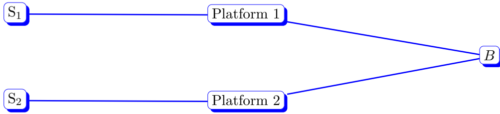
Figure 2: multi-homing
