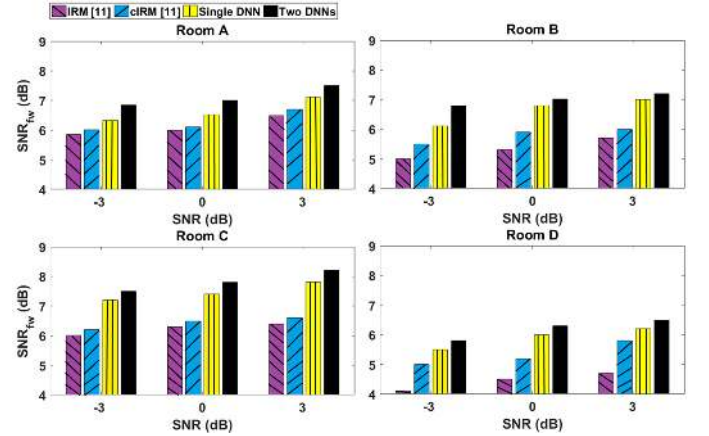
Fig. 9. The SNR fw (dB) in terms of different methods with various rooms i.e. different RT60s. The X-axis is the SNR level, the Y-axis is the SNR fw (dB), each result is the average value of 120 experiments. The interference is the undesired speech signal, respectively.
