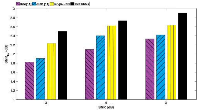
Fig. 11. The \text{SNR}_{fw} (dB) in terms of different methods with the unseen RIRs. The X-axis is the SNR level, the Y-axis is the \text{SNR}_{fw} (dB), each result is the average value of 120 experiments. The interference is the undesired speech signal, respectively.
