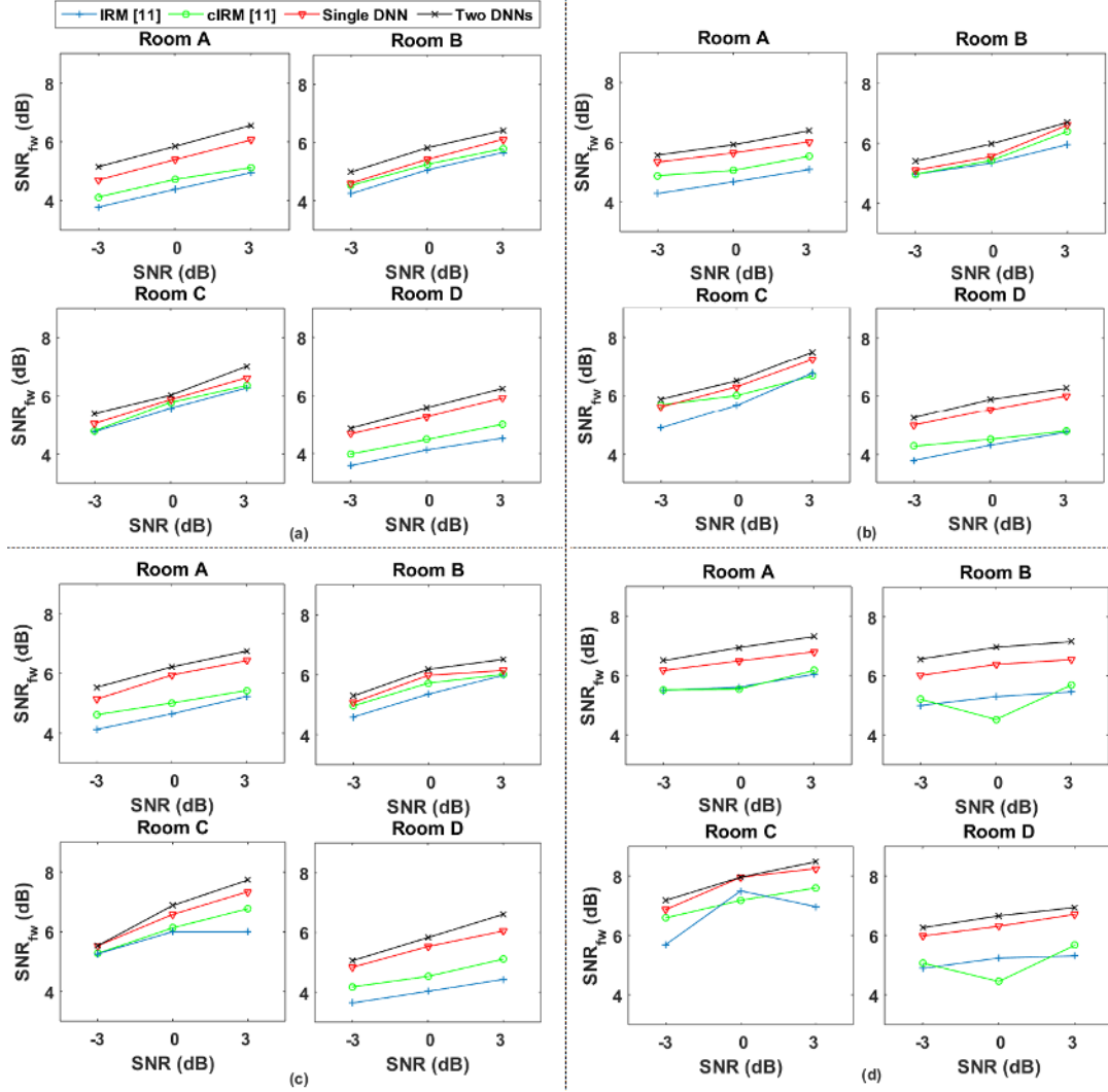
Fig. 5. The \text{SNR}_{fw} (dB) in terms of different methods with various rooms. The X-axis is the SNR level, the Y-axis is the \text{SNR}_{fw} (dB), each result is the average value of 120 experiments. The noise types in the subfigures (a), (b), (c) and (d) are factory, babble, cafe and SSN, respectively.
