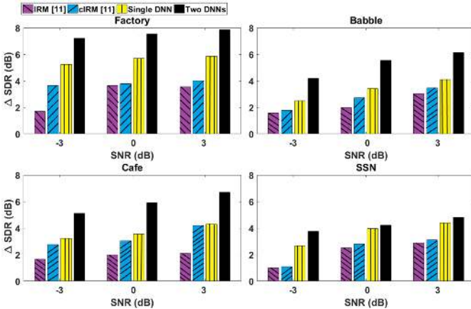
Fig. 8. The SDR improvement (dB) in terms of different methods with the unseen RIRs. The X-axis is the SNR level, the Y-axis is the SDR improvement (dB), each result is the average value of 120 experiments. The experimental results with four different types of noise are shown.
