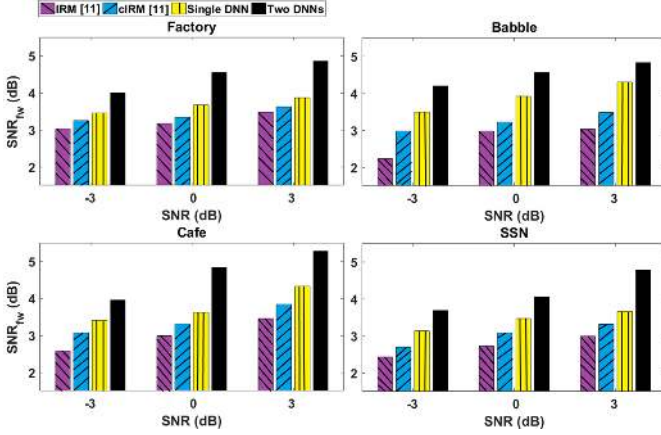
Fig. 7. The SNR fw (dB) in terms of different methods with the unseen RIRs. The X-axis is the SNR level, the Y-axis is the SNR fw (dB), each result is the average value of 120 experiments. The experimental results with four different types of noise are shown.
