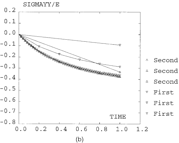
Figure 14. Extension and compression test, elastic analysis. Stress vs. time curves computed with the two algorithms (1, 5 and 50 time steps): (a) \sigma_{xx} , (b) \sigma_{yy}
