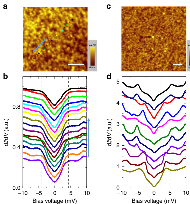
Fig. 4 Tunneling spectra measured on the smoother surface.
