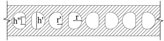
Fig. 9 Assumed section of the donut-type voided slab for calculating the moment of inertia.
