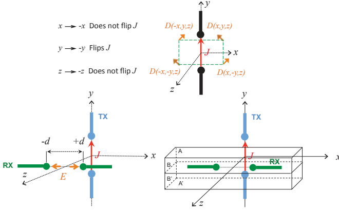
Fig. 5: Par-wise symmetrical antennas with input current ( I ) in the y -axis direction. Net energy flowing out the whole region around the RX antenna is zero which results in S_{12} = S_{21} = 0 .
