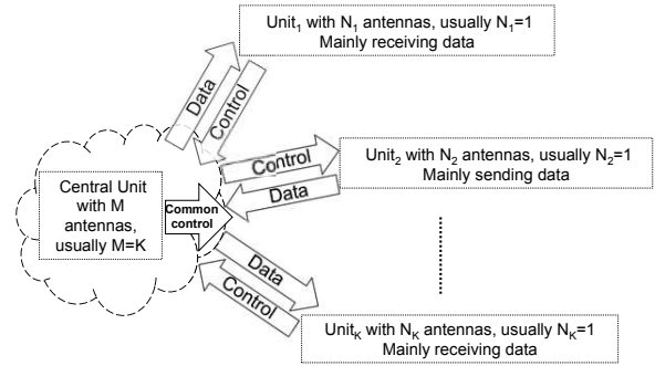
Fig. 1: 2K pipes of data/control are established over the same time/frequency where control includes reference for time/frequency/clock synchronization, channel gain/phase, information for user selection and channel inversion in SDMA, channel matrix in MIMO, ARQ, power control, instruction for adaptive coding and modulation, etc. In SDMA down-link, main data flow is out of central unit, while in SDMA uplink most data flow is into the central unit. Common control includes reference for time/frequency/clock synchronization.
