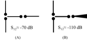
Fig. 9: Shape of arms is adjusted to compensate the lack of symmetry in a low coupling structure.
