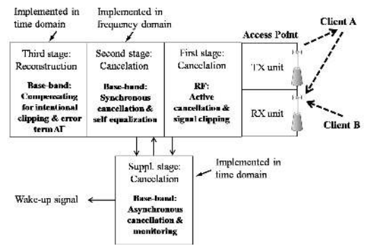
Fig. 4: Self-interference cancellation stages at an access point with a supplemental stage to support new clients in an asynchronous manner.
