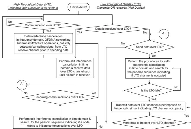
Fig. 11: Flow chart for superimposed networking.
