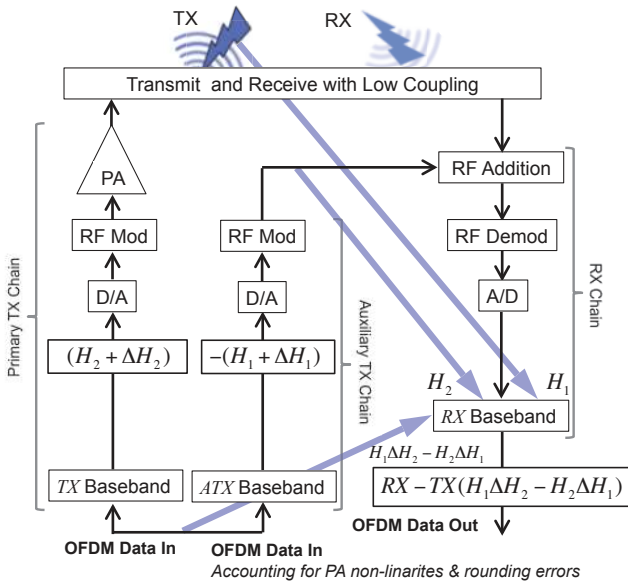
Fig. 3: Details of the self-interference cancellation.
