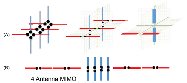
Fig. 7: Two and Three-dimensional antennas for MIMO structure.
