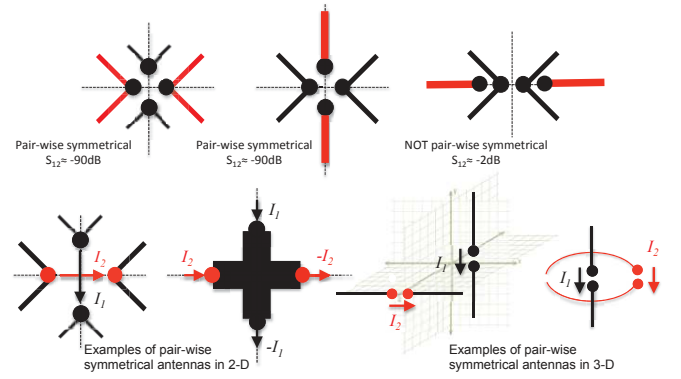
Fig. 6: All structures are pair-wise symmetric except for the one on top right corner which shows significant coupling.
