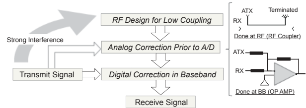
Fig. 2: Main components involved in self-interference cancellation.
