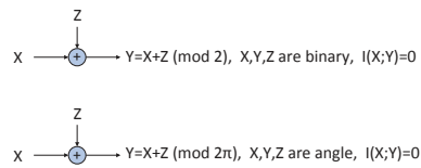
Fig. 14: Masking through modulo addition of phase values for unconditional security. Phase masks are obtained through measuring the channel between the legitimate parties at both ends. The number of transmissions to perform this measurement is limited and is done in a manner that eavesdropper encounters one unknown phase corresponding to each of its receive antennas (phase between eavesdropper receive antenna and antenna of the legitimate transmitter). Each shared phase value will be used to mask a PSK transmission, containing some of the bits of the final key. Errors between the measured phase values at the two legitimate parties will be part of errors observed in traditional systems and will be corrected by the underlying error correcting code.
