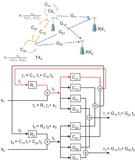
Fig. 10: R_1 and R_2 are filters at receivers of nodes TX1 and TX2, respectively. These filters superimpose a signal on the direct path which will cancel the interference from the cross links. Stability condition is satisfied by adjusting TX/RX gains.
