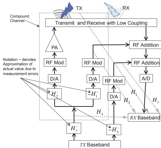
Fig. 16: Block diagram for cascade of analog cancellation. This enhances the ability for cancellation of self-interference through time domain filtering, and consequently, can be used to avoid delay (typical of OFDM) in closing the loop between legitimate parties in a key exchange protocol.
