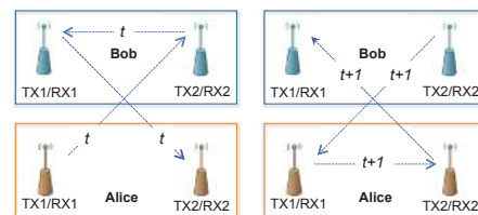
Fig. 15: Steps in key exchange: 1- At time t - 1 , Alice and Bob measure their loop-back channels from Bob/TX1 to Bob/RX2 and from Alice/TX2 to Alice/RX1 (send low power pilots after scrambling and loop back in each unit). 2- At time t , Alice/TX1 sends pilots (after scrambling) to Bob/RX2, who (using Bob/TX1) forwards it to Alice/RX2. 3- At time t + 1 , Bob/TX2 sends pilots (after scrambling) to Alice/RX1, who (using Alice/TX2) forwards it to Bob/RX1. 4- The two units, knowing their loop-back channels and relying on reciprocity, compute the channel: (\text{Alice/TX1 to Bob/RX2}) \times (\text{Bob-loop-back}) \times (\text{Bob/TX1 to Alice/RX2}) to be used as a key. This is possible as up/down conversion at each unit is performed using the same carrier/clock.
