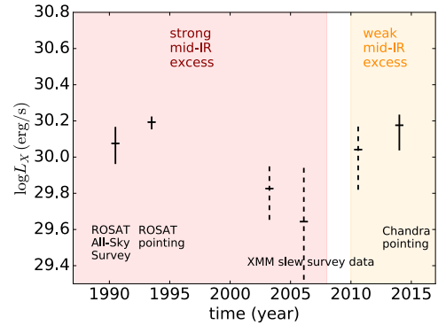
Fig. 2. Observed X-ray luminosity of TYC 8241 2652 1 is constant since 1991 with measurements before 1995 performed by ROSAT and the new measurement we report on here performed by Chandra in 2014. The low signal-to-noise detections achieved by the XMM-Newton slew survey from 2003 to 2010, indicated with dashed lines, are roughly consistent in luminosity with previous and later X-ray observations.
