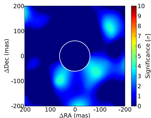
Fig. 4. Significance map derived by fitting a companion model to our NACO L' -band SAM data. All structures in the map have a significance \leq 4\sigma in the 40–250 mas range, which is consistent with a nondetection. The white inner circle represents our effective inner working angle with observations inside this annulus strongly adversely affected by S/N effects represented by limited contrast sensitivity.
