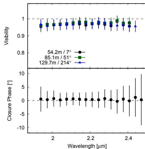
Fig. 3. Visibilities (top) and closure phases (bottom) extracted from our VLTI/AMBER observations.
