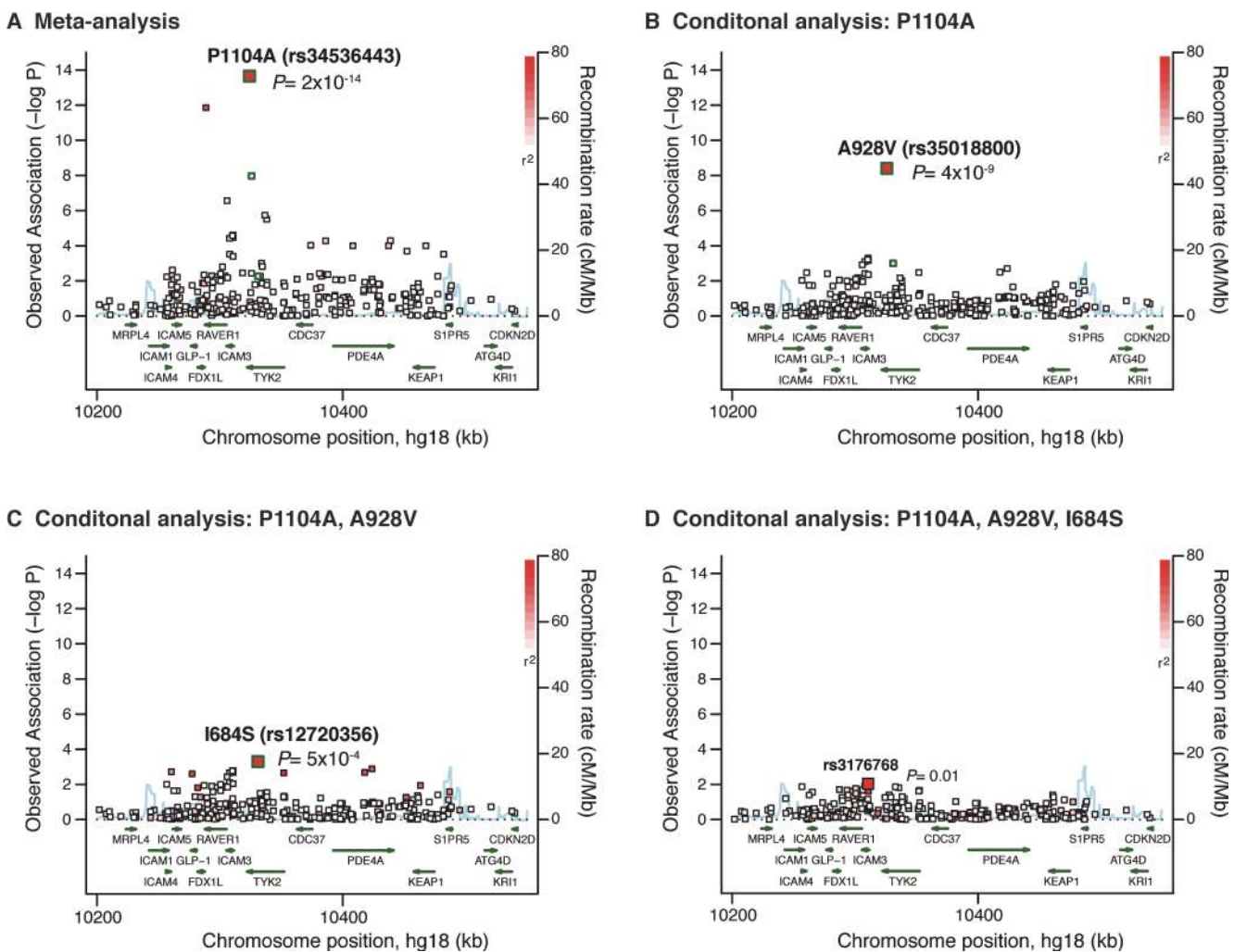
Fig 1. Results from stepwise conditional analysis of the TYK2 locus. We fine-mapped the TYK2 locus using ImmunoChip data available for 7,222 ACPA+ RA cases and 15,870 controls (MAF > 0). (A) In the meta-analysis, the best signal of association was at the TYK2 missense variant P1104A (rs34536443). (B) Conditional on P1104A, the best signal of association was at the TYK2 missense variant A928V (rs35018800). (C) Conditional on P1104A and A928V variants, the best signal of association is at the TYK2 missense variant I684S (rs12720356). (D) Conditional on the 3 RA-protective variants in TYK2 , we observed no additional signal of association at the locus (best signal is rs3176768, P = 0.01 ). P-values from meta-analyses of logistic regressions results from 6 ImmunoChip collections are shown. The three TYK2 missense variants predicted to be damaging and independently associated with RA risk are highlighted in green.
