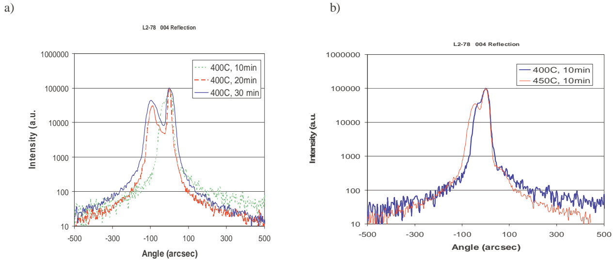
Figure 3. Thermal study of a \text{Al}_{0.3}\text{In}_{0.7}\text{AsSb} digital alloy film at (a.) 10-30 minutes at 400°C, and (b) 10 minutes at 400°C and 450°C.
