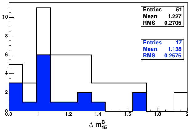
Fig. 8. Distribution of the light curve shape parameter \Delta m_{15}^B for the whole published set (51 SNe, white histogram, upper box) and the reference sample of 17 supernovae we selected (blue histogram, lower box).
