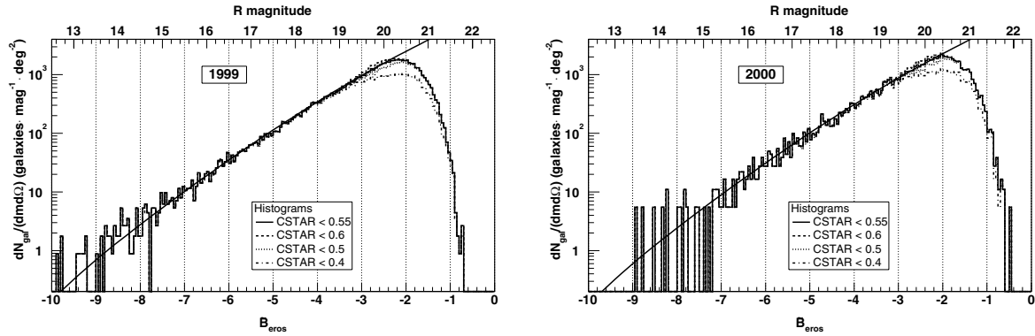
(a) Galaxy count on EROS fields done on 180 images from the 1999 search. The completeness limit is for \text{CSTAR} < 0.55 and \tilde{B}_{\text{eros}} < -2.6 .
