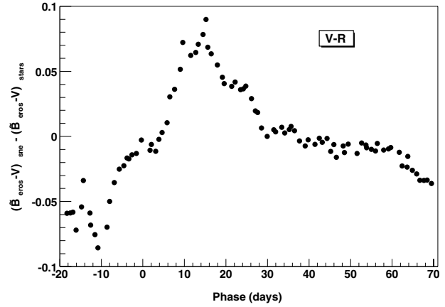
Fig. 9. Evolution with the supernova phase of the error we made when using stars to calibrate supernovae. What is actually plotted is the difference between zero points computed for SNe Ia (\overline{\mathcal{B}}_{\text{eros}} - V)_{\text{sne}} and for stars (\overline{\mathcal{B}}_{\text{eros}} - V)_{\text{stars}} . Each dot stands for a star whose color ( V - R ) is equal to the (V - R) color of a SNIa at that phase. The signal difference is never larger than 8%. The colors are computed from template spectra.
