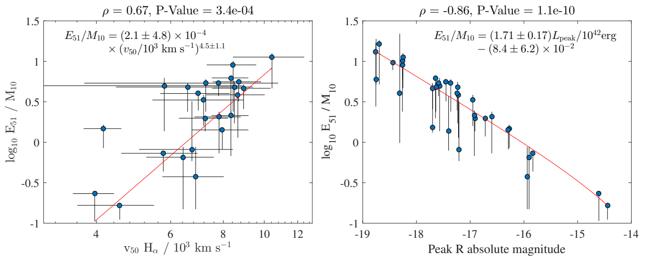
Figure 7. Left: E/M from the fit to RW11 as a function of the velocity normalized to v_{50} of H_{\alpha} . Right: E/M from RW11 as a function of peak magnitude. Red lines are the best fits described in the text.
