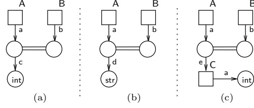
Fig. 10. Three patterns with is edges
