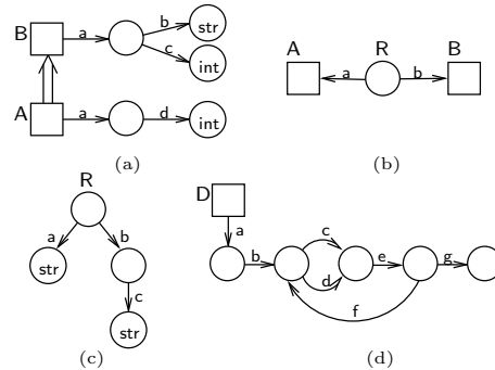
Fig. 4. Simulating other data models
