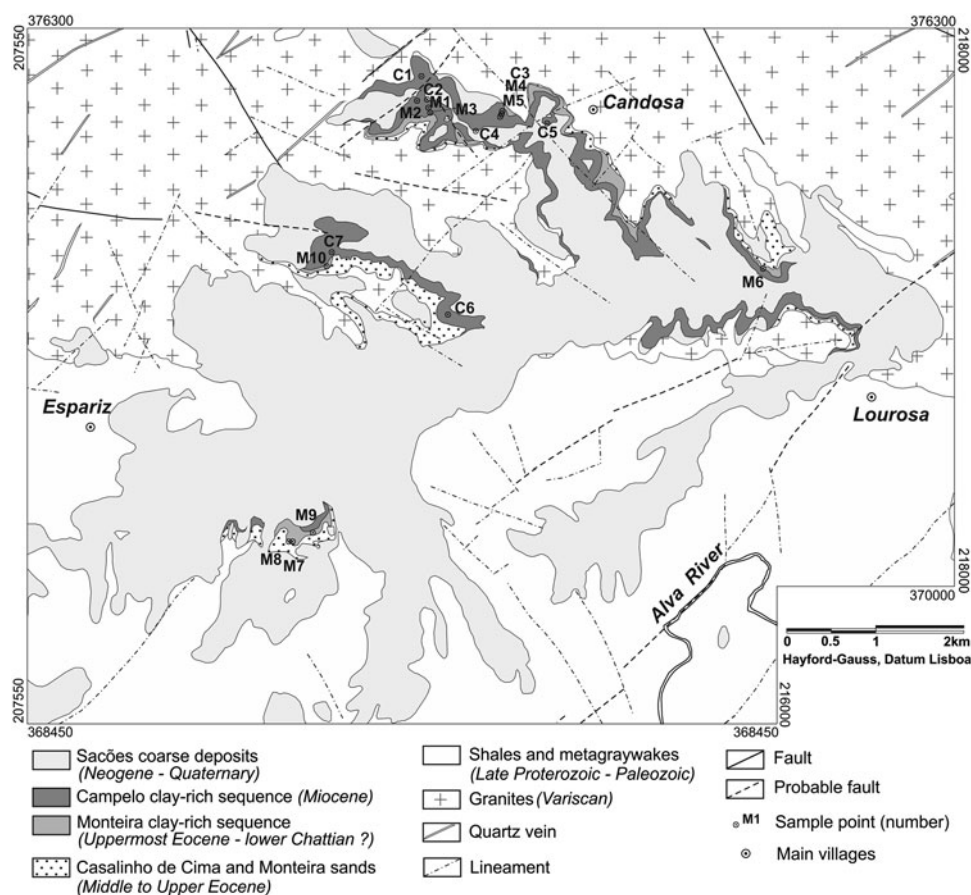
Fig. 2 Map of clay resources in the Tábua region and sample points location
