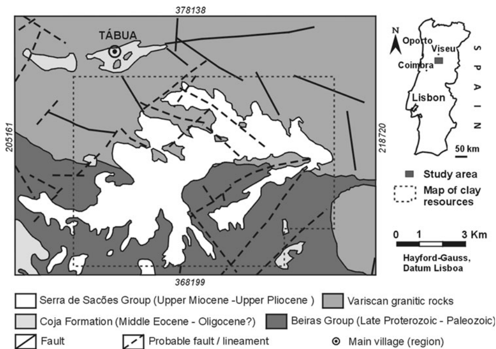
Fig. 1 Geological map of the study area (modified from Cunha 1992)
