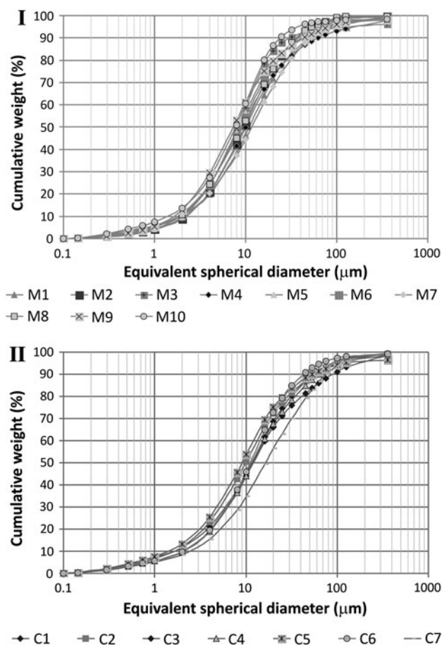
Fig. 3 Grain-size cumulative curves of the samples collected in Tábua region. I - Monteiro group; II - Campelo group
