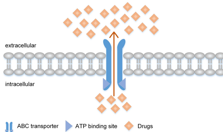
Fig. 1 ABC transporters decrease intracellular drug concentration conferring MDR. Cancer cells promote overexpression or activation of ABC transporter, enhancing the efflux of chemotherapeutic drugs, which leads to a lower intracellular drug concentration and results in MDR phenotype
