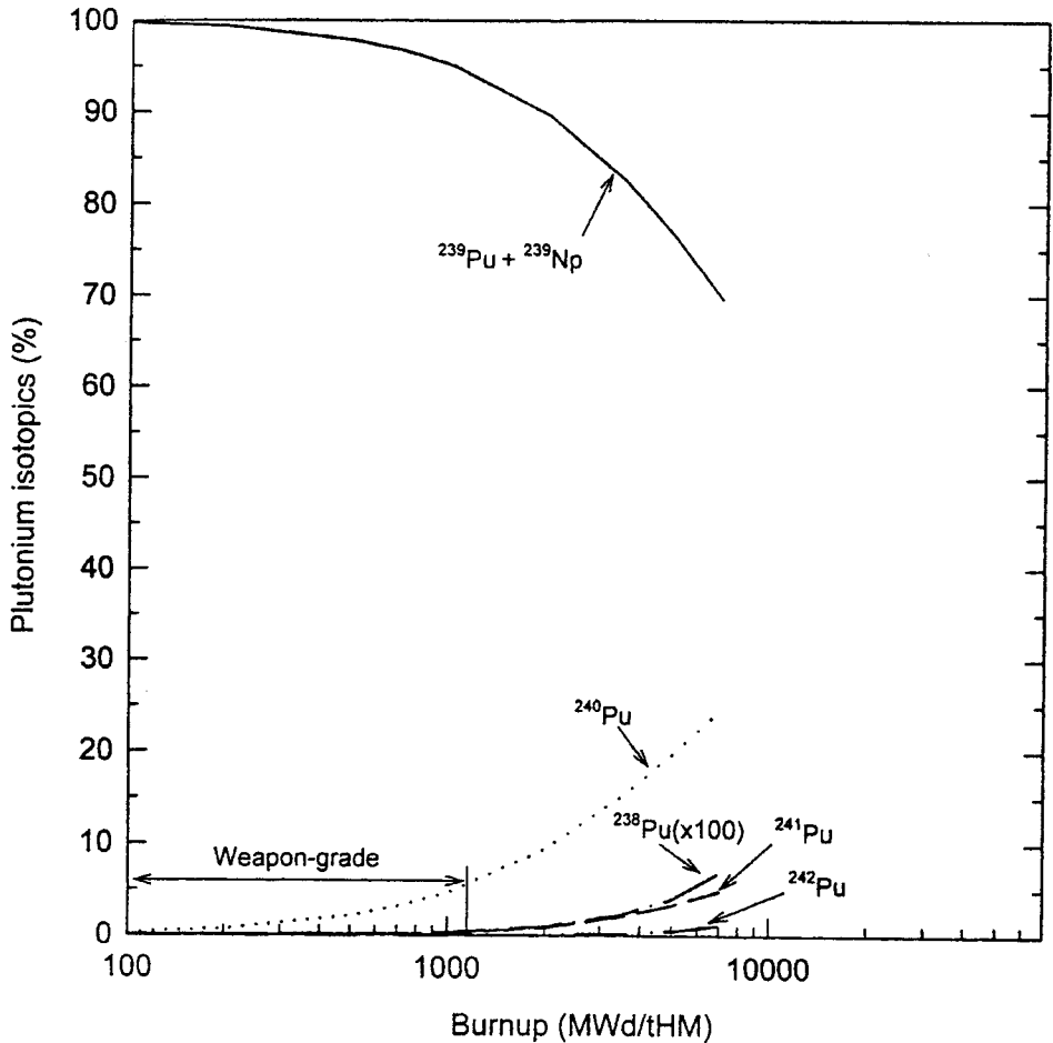
Figure 11a: Plutonium isotopics as a function of burnup in a natural-uranium fueled heavy-water reactor.
