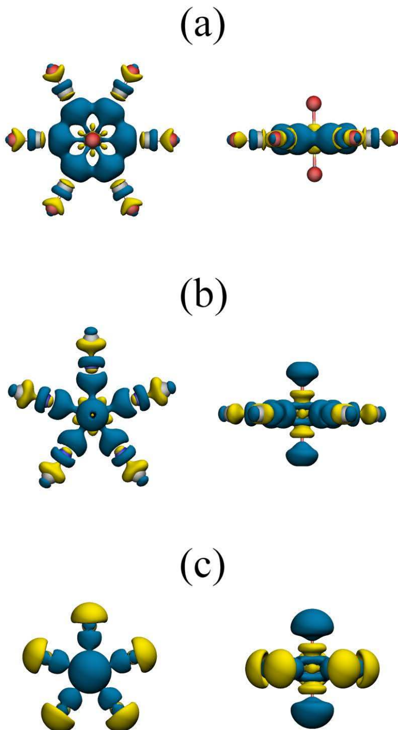
Figure 2. Density difference plots of the a) carbonyl, b) isocyno and c) fluoro complexes of uranyl, calculated by subtracting the TPSSh-calculated electron densities of the uranyl and
