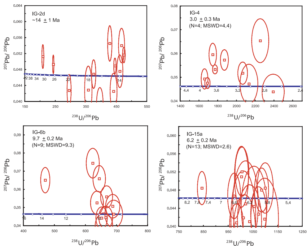
Fig. 7. Tera-Wasserburg concordia diagrams showing U-Pb SHRIMP ages for group A samples – from within the Namche Barwa massif. Error ellipses are shown at 2\sigma uncertainty. Older zircon core ages are shown, where applicable, for all samples on composite Concordia plot.
