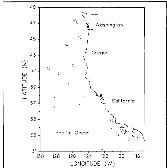
Figure 1. Sightings of mesoplodont beaked whales off California, Oregon and Washington based on aerial and shipboard surveys, 1975-1993 (data from Dohl et al. 1980, 1983; Green et al. 1992, unpublished data; Hill and Barlow 1992; Carretta and Forney 1993; Mangels and Gerrodette 1994; NMFS, unpublished data).
