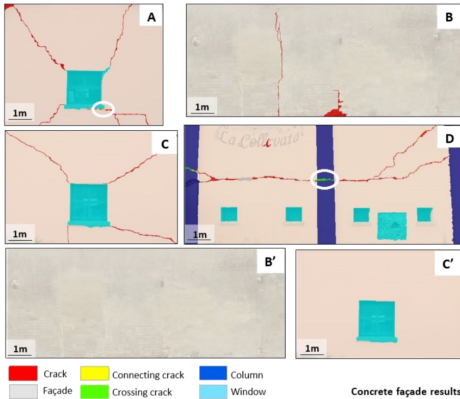
Figure 8. Results of applying the concrete rule set on six concrete façade. (b') and (c') were edited in order to remove the damage feature. (a) and (d) highlight cases of connecting and crossing cracks. (a) highlights with a circle the location of a connection, the small nature of a crack connecting with a window makes it hard to visualize it in the illustration. (d) illustrates a crack crossing a column as a green object (highlighted by circle). Scale approx.
