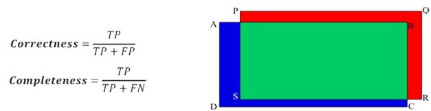
Figure 5. Equations for the correctness and completeness accuracy measurements based on the accuracy indicator: false positive (FP, red), false negative (FN, blue), and true positive (TP, green) (Joshi, 2010).
