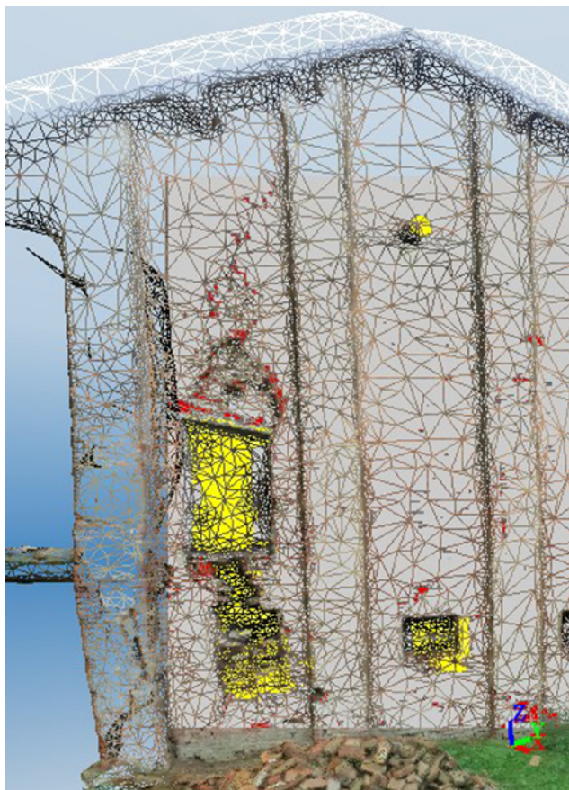
Figure 13. Example of the wire mesh with OBIA extracted information overlaid. Yellow indicated holes, and red indicated cracks in the façade (for better contrast, the color scheme was changed from the previous examples).
