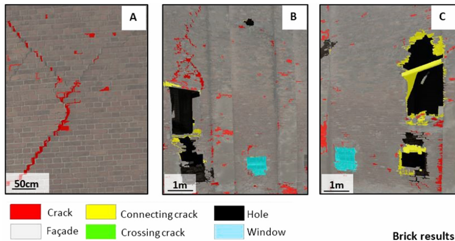
Figure 9. Results of applying the brick rule set on three brick façade images. Scale approx.
