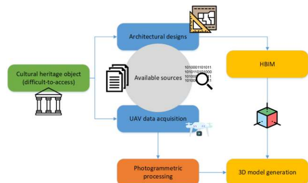
Figure 3: Workflow of the BIM generation of Averof’s Museum, Metsovo, Greece
