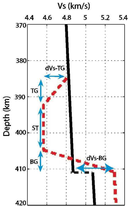
Figure 9. Double gradient slab (DGS) model parameterization. The IASPI91 velocity model is indicated by the solid black line with an example DGS velocity model indicated by the dashed red line. The five model parameters are TG, top gradient thickness (km); ST, constant velocity slab thickness (km); BG, bottom gradient thickness (km); dV_s -TG, shear wave velocity decrease for top gradient (km/s); and dV_s -BG, shear wave velocity increase for bottom gradient (km/s). The value of dV_s -BG is the velocity increase with respect to the IASPI91 model value immediately above the 410-km velocity step.
