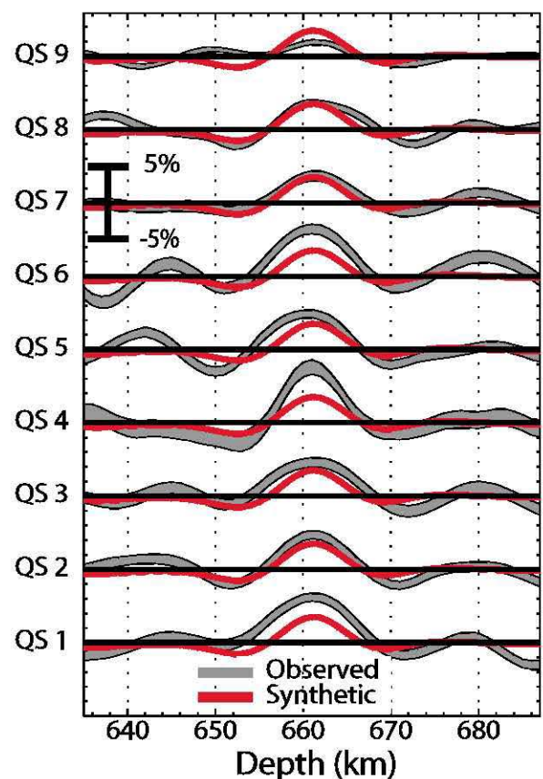
Figure 16. Observed and synthetic 660-km discontinuity arrivals. The vertical scale shows an amplitude range of 10% relative to vertical P wave arrival. The gray swath is the one-sigma bounds of the observed signal, and the red lines are the IASPI91 velocity model predictions for a mean ray parameter of our data set (0.06 s/km). The pulse widths of the observed and synthetic data are similar, although the observed amplitudes are generally higher than IASPI91 predictions.
