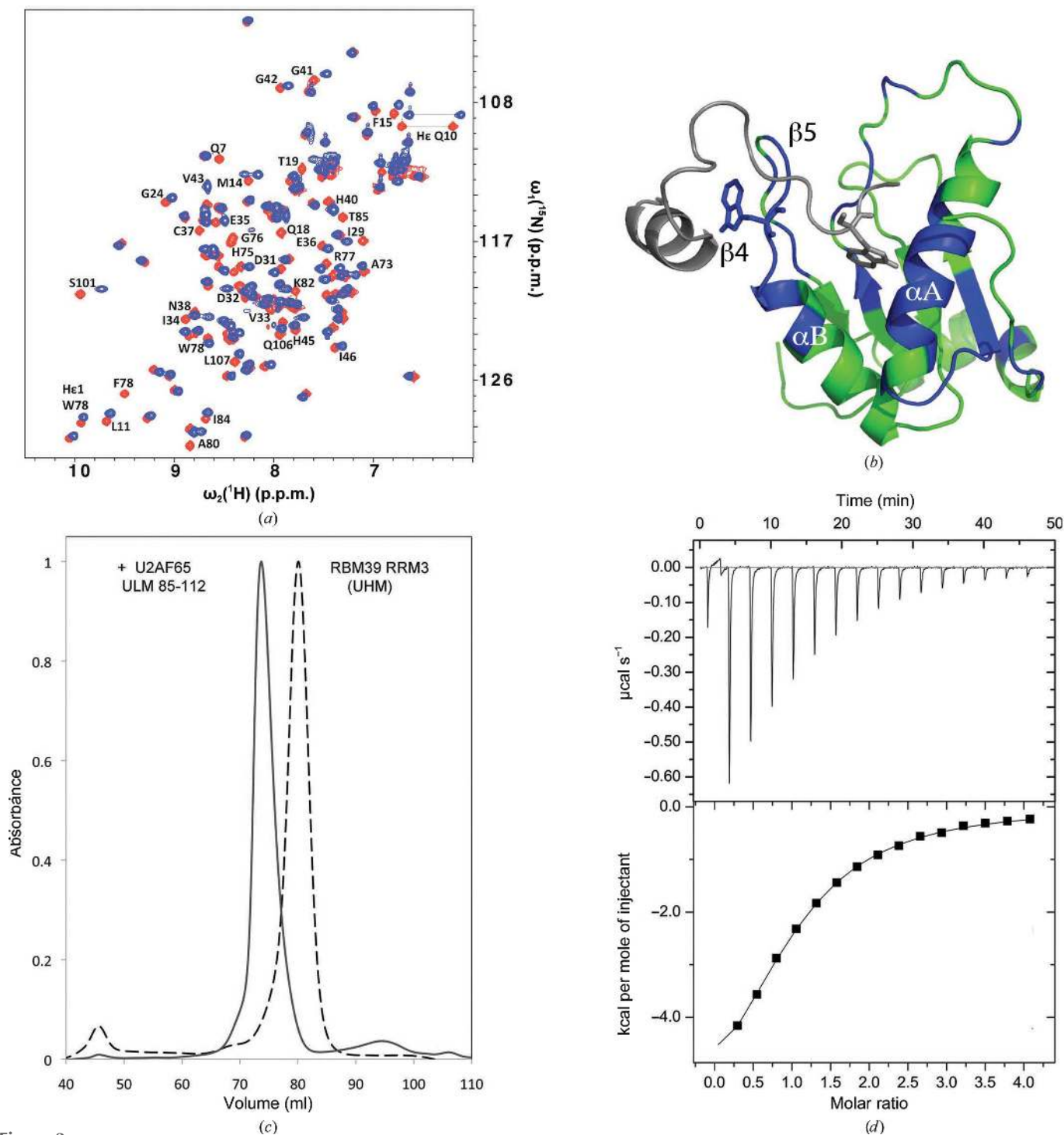
Figure 3 Biochemical analysis of RBM39-UHM-U2AF65-ULM interactions. (a) Superposition of the two-dimensional [^{15}\text{N},^1\text{H}] -HSQC spectra of ^{15}\text{N} -labeled RBM39-UHM in the absence (red) and presence (blue) of 1.3 equivalents of unlabeled U2AF65-ULM (residues 85–112). The resonances of residues with chemical shift changes of \geq 0.13 p.p.m. are labeled. (b) Model of the RBM39-UHM-U2AF65-ULM complex generated by HADDOCK . The NMR structure of RBM39-UHM (color-coded as described below) was used as the input, and the U2AF65-ULM fragment (gray) was docked to it using NMR constraints derived from the chemical shift mapping. RBM39-UHM residues experiencing either large chemical shifts, line broadening and chemical shifts, or broadening beyond detection are colored blue, while those with no significant changes are colored green. The reciprocal tryptophans are shown as stick diagrams. (c) Normalized size-exclusion chromatography elution profiles of RBM39-UHM and a mixture of RBM39-UHM and U2AF65-ULM (residues 85–112) in a 1:2 molar ratio. (d) Isothermal titration calorimetry profile of solutions of RBM39-UHM and the U2AF65-ULM (85–112) peptide, showing binding with a K_d of 20 \mu\text{M} .
