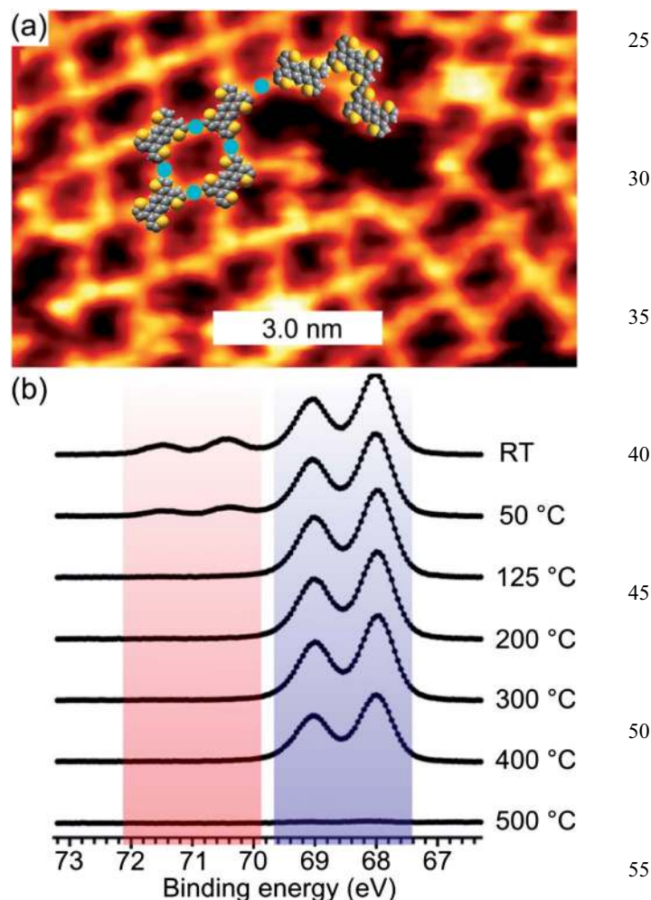
Fig. 5 (a) STM image of the 2D network on Ag(111) ( U_{\text{bias}} = -758 mV, I_{\text{tunnel}} = 0.877 nA). (b) Core level spectra of the Br 3d level on Ag(111) at room temperature and various annealing temperatures up to 500 °C.
