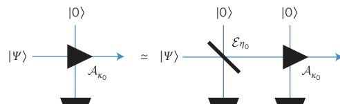
Figure 3 | Graphical representation of equation (6). The symbol ‘ \simeq ’ indicates that applying the quantum-limited amplifier \mathcal{A}_{\kappa_0} to pure input |\psi\rangle or to its evolved counterpart via a lossy channel of transmissivity \eta_0 = 1 - 1/\kappa_0 (that is, \mathcal{E}_{\eta_0}(|\psi\rangle\langle\psi|) ) produces outputs that have the same spectra.
