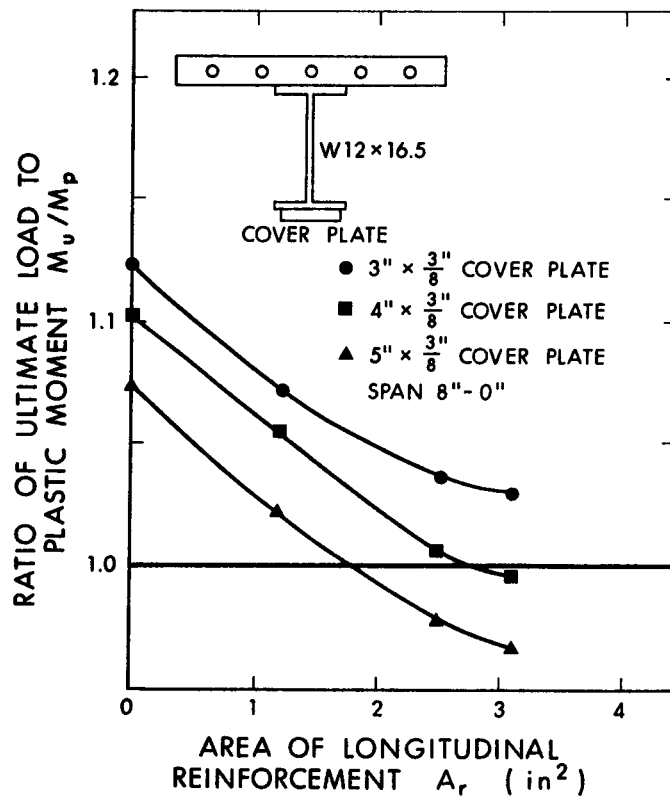
(b) EFFECT OF AREA OF LONGITUDINAL REINFORCEMENT ON M_u/M_p RATIO
