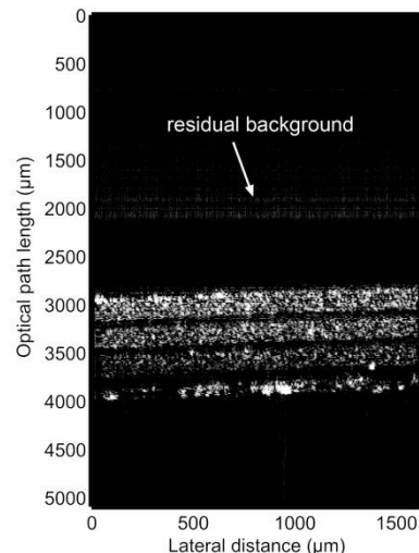
Fig. 3. OCT cross-sectional image (average of 100 B-scans) of a layered tissue phantom.
