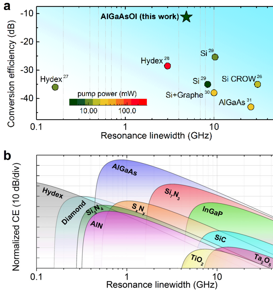
Figure 6 CW-FWM performance comparison for microresonators
