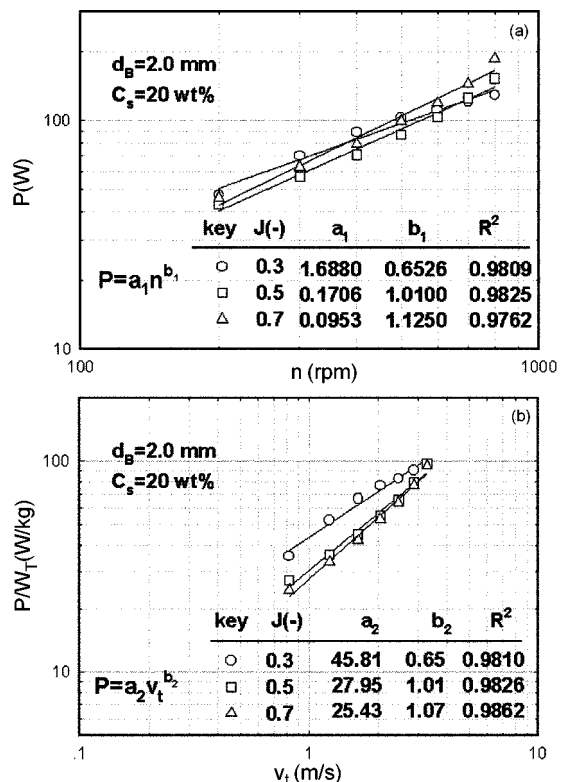
Fig. 2. (a) The effect of rotation speed and ball filling ratio on power input. (b) The effect of peripheral velocity of stirrer and ball filling ratio on power input.
