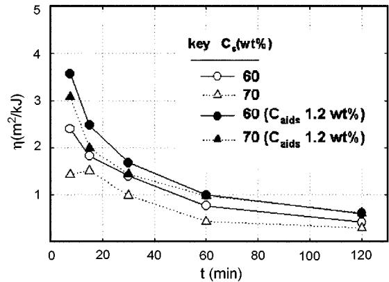
Fig. 10. \eta vs. t for exp. conds(Exp. conds.: n=700 rpm, J=0.7 , d_B=1.0 mm).
