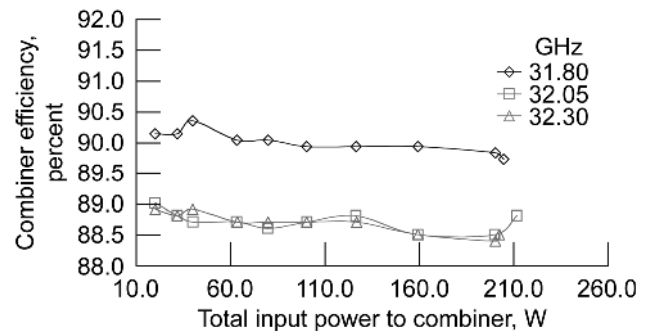
Figure 4.—Measured efficiency of magic-T based power combiner as function of total input power.
