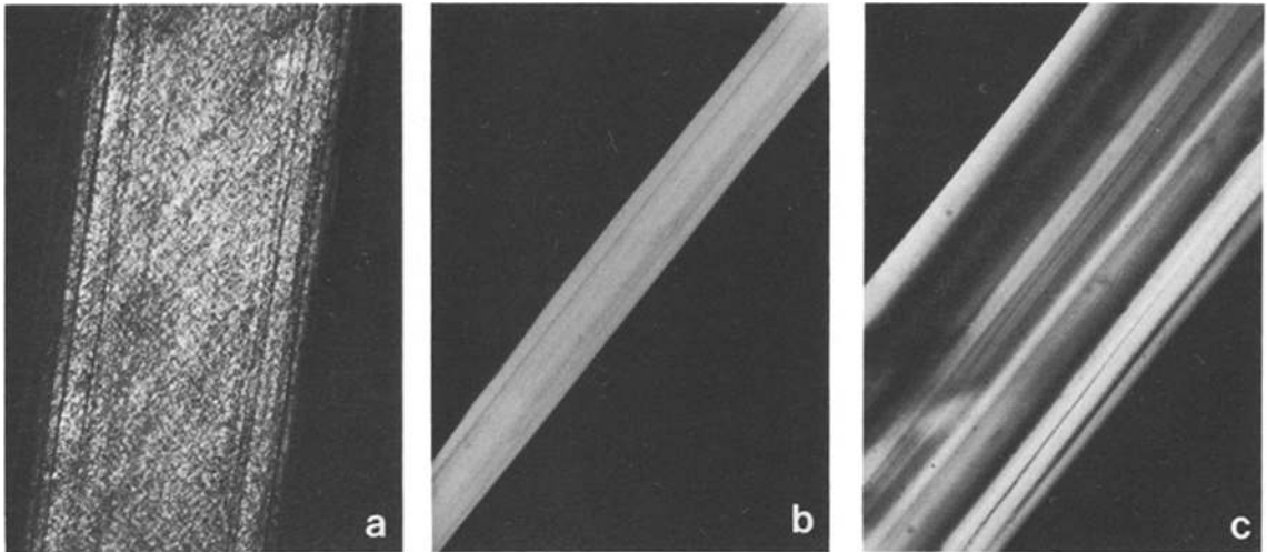
Figure 11 Optical micrographs of polyethylene fibres. Crossed Nicols. a draw ratio 1, magnification 96 \times ; b draw ratio 25.5, magnification 120 \times ; c draw ratio 25.5, magnification 480 \times .
