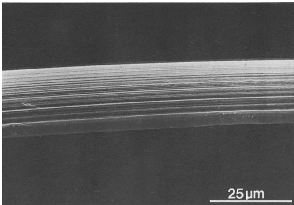
Figure 12 Scanning electron micrograph of a 31.7 times drawn polyethylene fibre.
