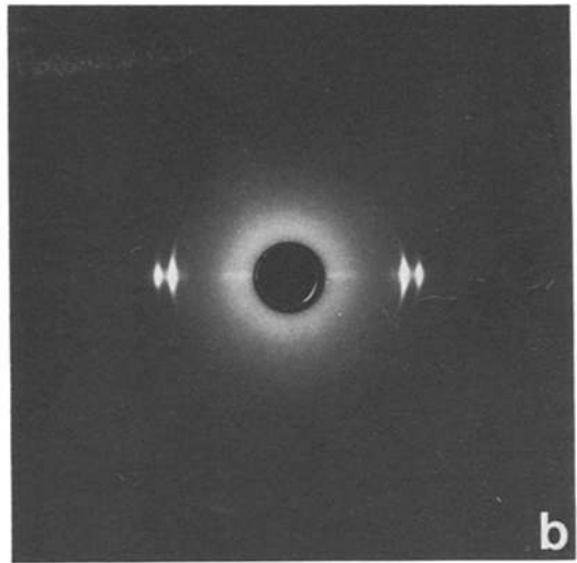
Figure 13 WAXS-patterns of drawn polyethylene filaments. Draw ratios: a 1.5; b 15.7; c 31.7. Fibre axis vertical.
