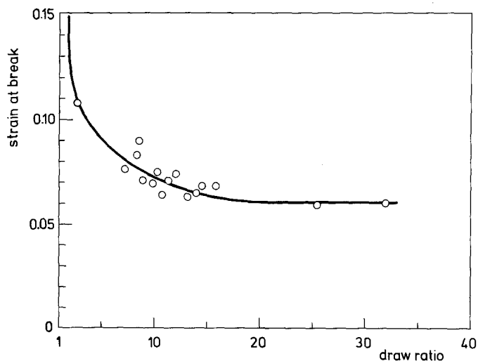
Figure 8 Dependence of the strain at break on the draw ratio.
