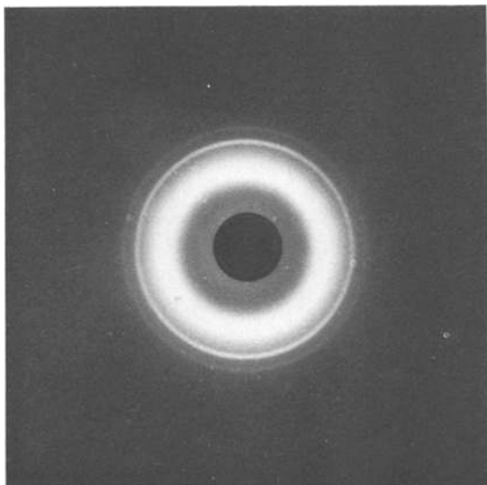
Figure 4 WAXS-pattern of polyethylene/decalin gel.
