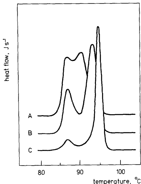
Figure 2 DSC-heating thermograms of polyethylene/decalin gel. Scan speeds: A 40^{\circ}\text{C min}^{-1} ; B 20^{\circ}\text{C min}^{-1} ; C 5^{\circ}\text{C min}^{-1} .
