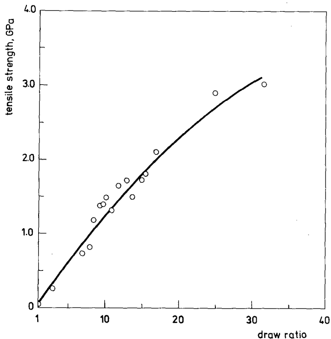
Figure 7 Tensile strength versus draw ratio of polyethylene filaments.
