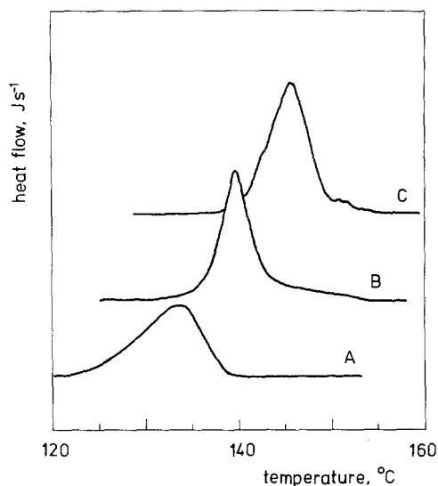
Figure 9 DSC-heating thermograms of solution-spun/drawn polyethylene fibres. Scan speed 10^{\circ}\text{C min}^{-1} . Draw ratios: A 1; B 15.7; C 31.7.
