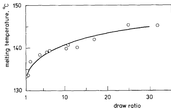
Figure 10 DSC-(peak)melting temperatures versus draw ratio of polyethylene monofilaments.
