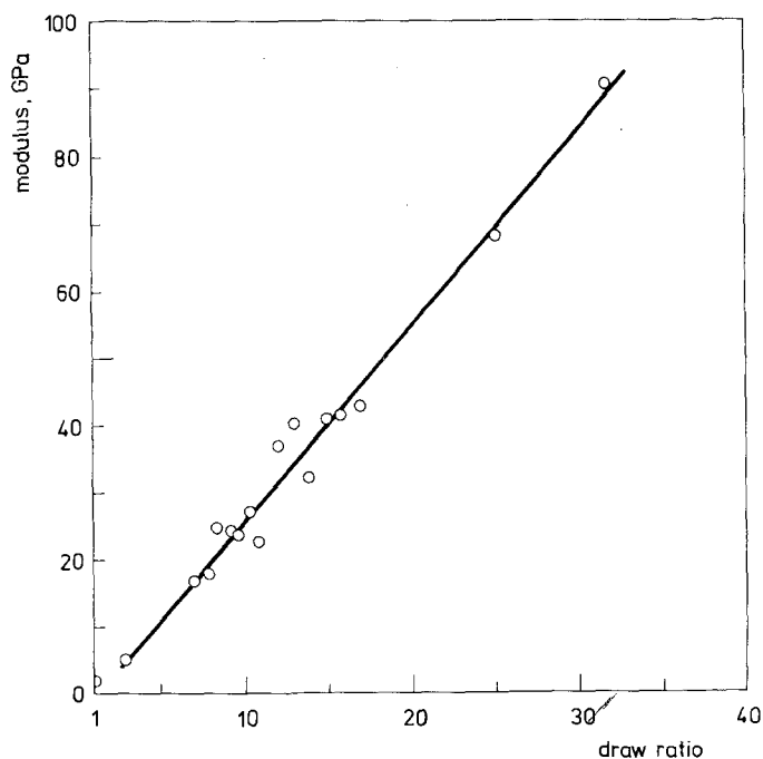
Figure 6 Young's modulus—drawn ratio relationship of polyethylene filaments.
