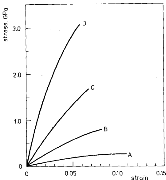
Figure 5 Stress-strain curves of solution-spun/drawn polyethylene fibres. Draw ratios: A 2.8; B 8.4; C 15.7; D 31.7.
