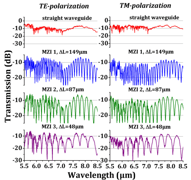
Fig. 2. Transmission measurements in TE and TM polarizations for 9.4 mm-long waveguide and asymmetric MZIs. The reported transmissions include coupling losses in/out of the chip. Red line shows the transmission of the straight waveguide. Blue, green, and purple lines represent the transmission of MZIs with arm difference of: 149 \mu\text{m} , 87 \mu\text{m} and 48 \mu\text{m} respectively. The transmissions are plotted separately to better highlight the spectral features.
