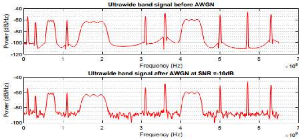
FIGURE 15. Chirp Signals Spread Across The Entire Frequency Spectrum.
