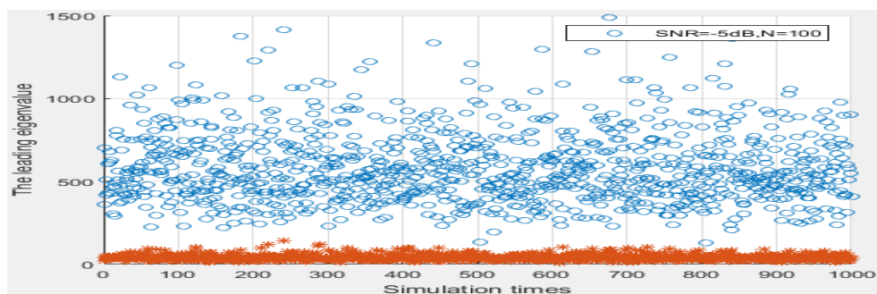
FIGURE 4. Statistics Realization Distance Between Signal and Noise [2]
