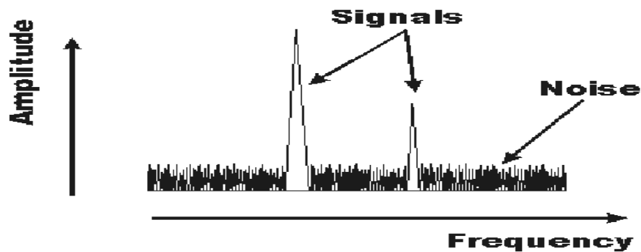
FIGURE 2. Noise and Amplitude Range of an FFT of Signal x(t)
