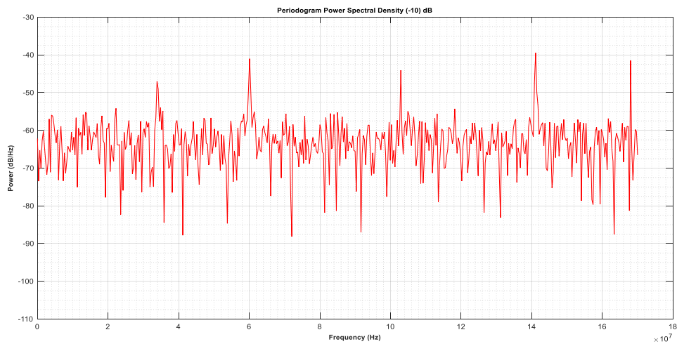
FIGURE 8. Graph of Periodogram Power Spectral Density with Noise
