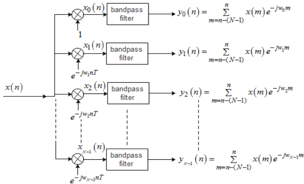
FIGURE 14. Decompose a Signal Into N=64 Sub-band Channels Using FFT
