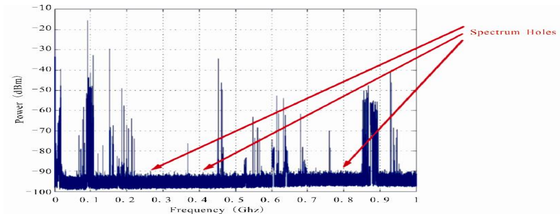
FIGURE 3. Measuring Spectrum Across a 900 kHz-1 GHz Band (Lawrence, USA) [4]
