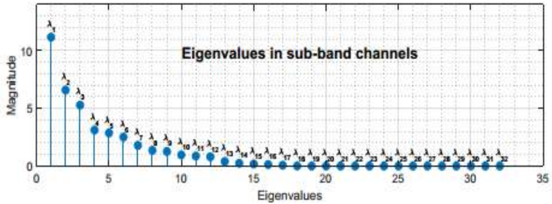
FIGURE 18. Principal Components with These Eigenvalues.
