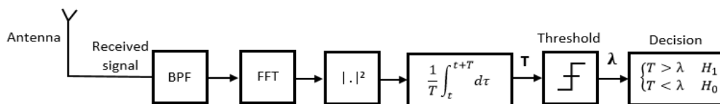
FIGURE 1. Energy Detection Model
