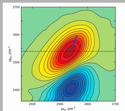
2D-IR spectrum at T_w = 0.2 ps. A dotted horizontal line defines a frequency slice at \omega_m = 2540 cm -1 along the \omega_\tau axis
