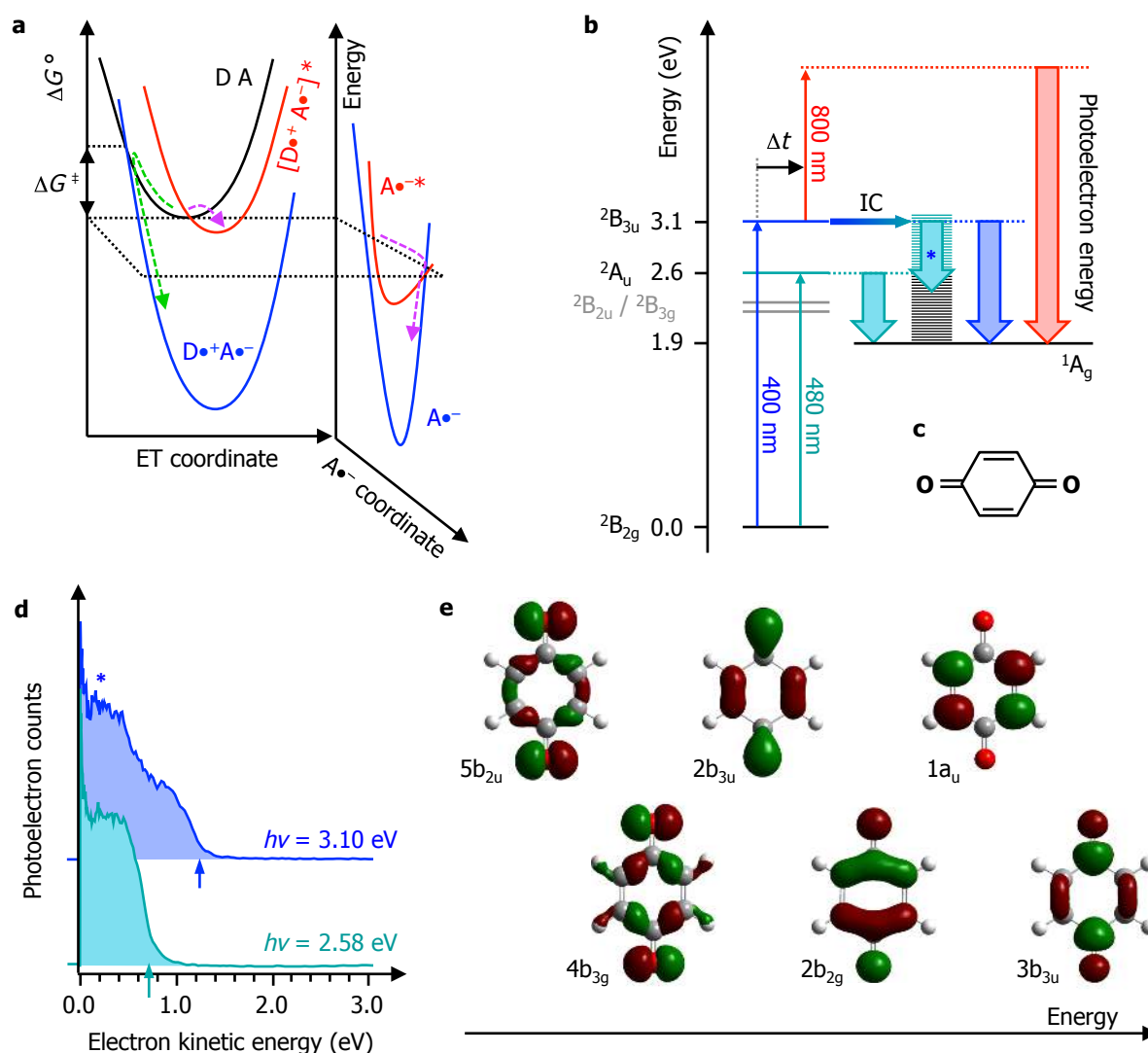
Figure 1 | Overview of electron transfer reactions and electronic structure of
