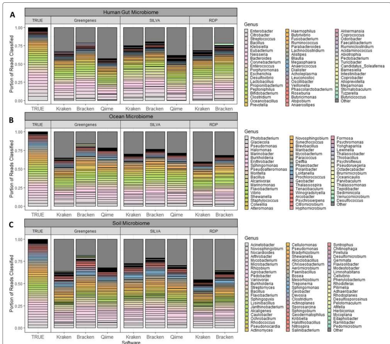
Fig. 2 Genera distribution for simulated microbiota. This plot compares the true genus relative abundances against those relative abundances estimated by Kraken, Bracken, and Qiime’s q2-feature-classifier, for each of the three simulated microbiome samples ( a human gut microbiome, b ocean microbiome, c soil microbiome). Only the correct genera are represented by different bars while read assignments to any incorrect taxon are included in “Other”
