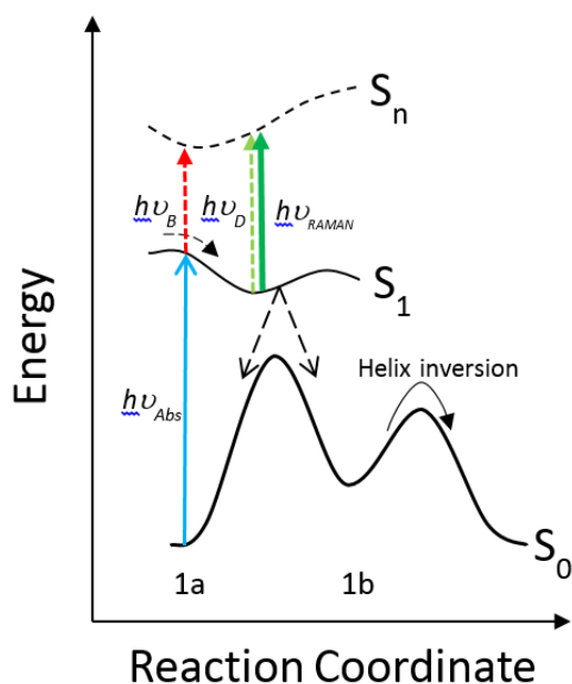
Figure 3. Schematic 1D plot of Energy as a Function of Reaction Coordinate. In this representation of the multidimensional reactive potential energy surface the Franck-Condon excited bright state absorbs at 760 nm. As structural relaxation occurs in 100 fs toward the dark state the S_1 energy decreases but the spectrum blue shifts, requiring increasing energy separation to S_n . The dark state is formed in 100 fs and absorbs at 550 nm. Its structure is significantly different to the bright state, such that the higher ( S_n ) excited state need not be of the same origin as for the bright state, and other intermediate states of lower transition moment may exist. As the dark state forms the S_0 energy increases and internal conversion to the ground state may occur at CIs. Note that the structural coordinate connecting bright and dark states need not be the same as that connecting the dark state to the CI and 1b .
