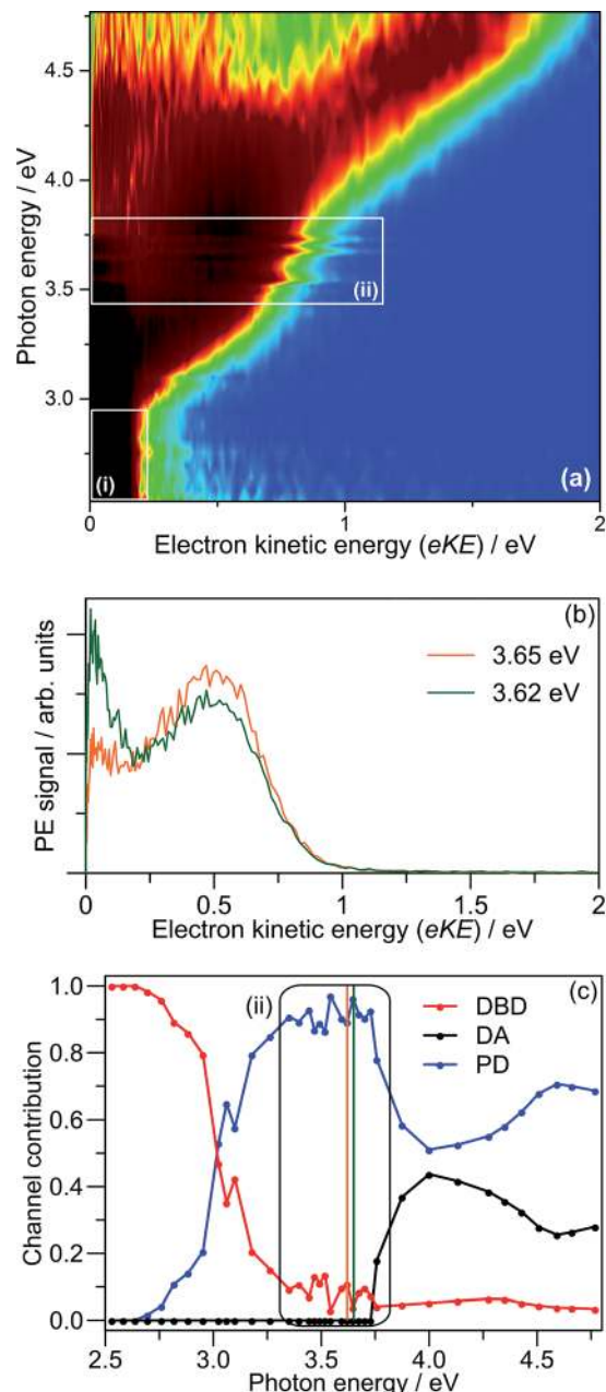
Fig. 3 (a) Frequency-resolved photoelectron spectra of (CQ_0)_2^- ; (b) two example spectra from region (ii); and (c) global fit contributions of each detachment channel from (a). The orange and green bars in (c) indicate the two spectra in (b).
