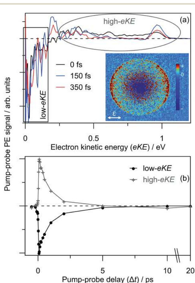
Fig. 8 3.10 + 1.05 eV time-resolved dynamics: (a) three example \Delta t spectra, which are divided a low-eKE and high-eKE contributions; and (b) integrated contributions of each the two pump-probe contributions. The 150 fs pump-probe velocity-map image is inset in (a), illustrating \beta_2 \sim +2 (relative to the polarisation, \epsilon ) for the high-eKE feature.
