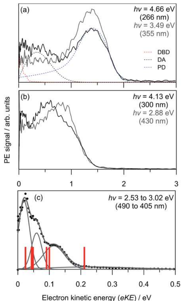
Fig. 2 Example (CQ_0)_2^- photoelectron spectra (black) and CQ_0^- (grey) from ref. 28 at three h\nu : (a) 4.66 eV; (b) 4.13 eV; (c) average between 2.53 eV and 3.02 eV. Included in (a) are the contributions from the three global-fit channels. The red bars in (c) are calculated carbonyl wagging modes localised on the non-planar monomer.
