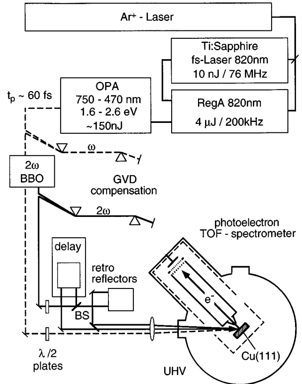
FIG. 3. Experimental setup.
