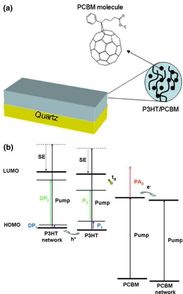
Fig. 1 a A schematic representation of the P3HT/PCBM blend materials on the quartz substrate. The zoom shows the morphology of this bulk heterojunctions and the arrow indicates the molecular structure of the PCBM. b Energy band diagram of blend materials for bound and mobile electrons and holes. The arrows P_1 and P_2 represent the localized polarons whereas the DP_1 and DP_2 represent the delocalized polarons, respectively. PA_3 represents the secondary excitation of free electrons in the PCBM and SE the stimulated emission
