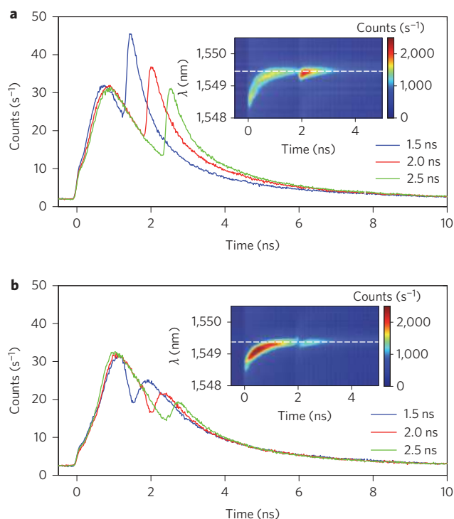
Figure 4 | Dynamic modulation of the SE decay curves at the target cavity. a , \mu PL decay curves at the wavelength indicated by a white dashed line in the inset, with different delay times of 1.5, 2.0, 2.5 ns of the control pulse. The inset shows a time-resolved \mu PL map at zero initial detuning. b , The same as a for an initial detuning of -0.6 nm.
