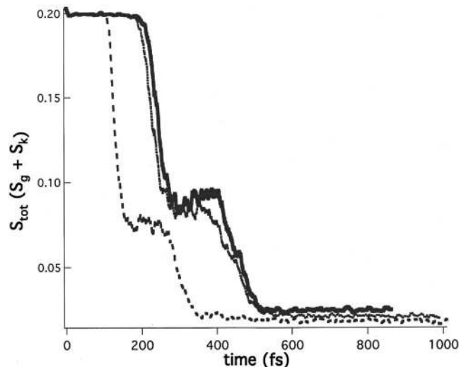
FIG. 2. Evolution of the tetrahedral order parameter as a function of time. The dashed curve corresponds to the BO_1 simulation and the solid curve to the BO_2 simulation. The dotted curve is the result from the CP simulation. The difference in the time scale to fully compress the simulation cell is dictated by the fictitious cell mass (see Table I). Graphite corresponds to a value of 0.2 and pure cubic diamond to a value of 0. A nonmartensitic transition to a liquid phase would have shown an increase in the value of the order parameter to 0.25 or greater, followed a monotonic decrease to 0.
