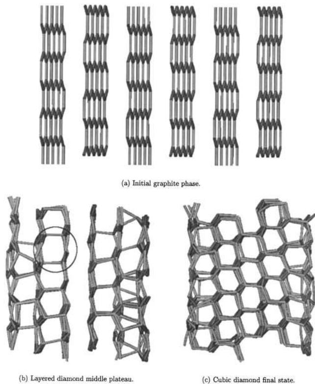
FIG. 4. Snapshots of the BO_1 simulation at various points during shock compression. The circled region in the layered diamond snapshot (b) corresponds to a likely hexagonal diamond region.
