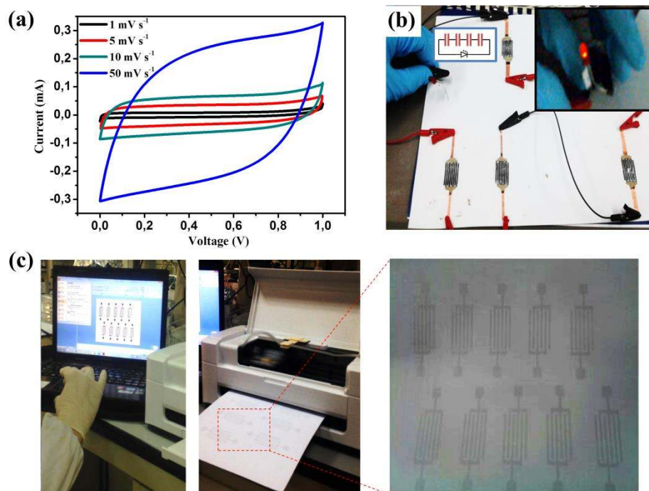
Figure 4. (a) Cyclic voltammetry curves of an EG/PH1000 hybrid ink (total amount 10 mL) MSC on a paper substrate at scan rates of 1 mV s -1 to 50 mV s -1 . (b) A charged MSC array containing 4 single devices can power an LED. (c) Inkjet printing of custom designed MSC arrays from a “home computer and printer” using pristine EG ink.
