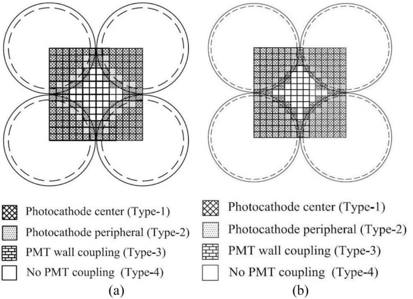
Fig.4. Crystal-to-PMT coupling regions. (a) 14 \times 14 animal PET and (b) 15 \times 15 human PET.
