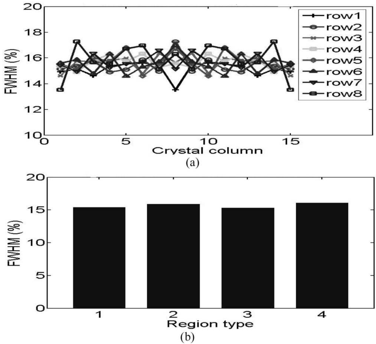
Fig.9. Energy resolution distribution of 15 x 15 LSO human PET detectors (a) Individual crystals. (b) Four coupling regions.
