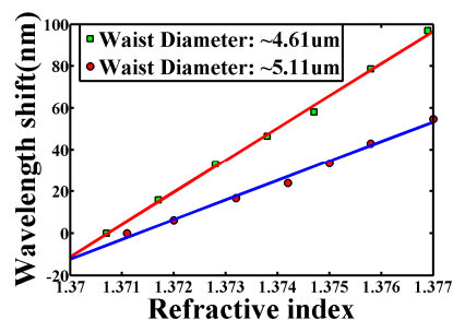
Fig. 5. Resonant wavelength shift as a function of RI: comparison for two different taper diameters.
