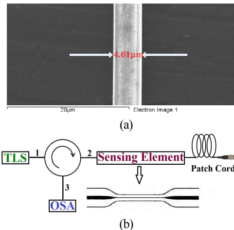
Fig. 2. (a) SEM image of the taper waist with a diameter of 4.61 \mu\text{m} and (b) experimental set-up of the refractive index sensor.
