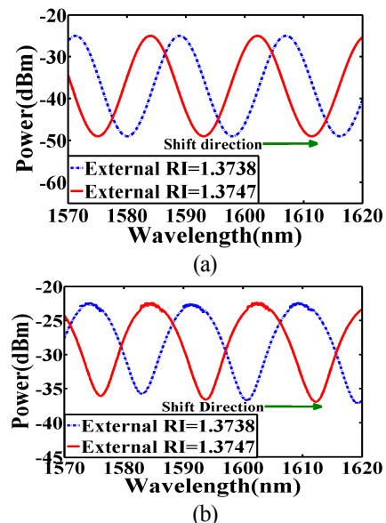
Fig. 3. (a) Calculated results and (b) experimental results of wavelength response of the microfiber sensor surrounded by different concentration of the salt solutions.
