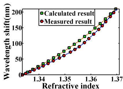
Fig. 4. Resonant wavelength shift as a function of RI: theoretical prediction and measured result for waist diameter \sim 5.11 \mu\text{m} .
