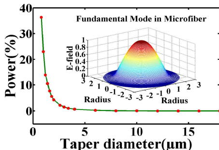
Fig. 1. Plot of optical power coupling out of a microfiber against different taper diameter. The inset shows the E-field profile of fundamental mode of a microfiber with a taper waist diameter of 4 \mu\text{m} .
