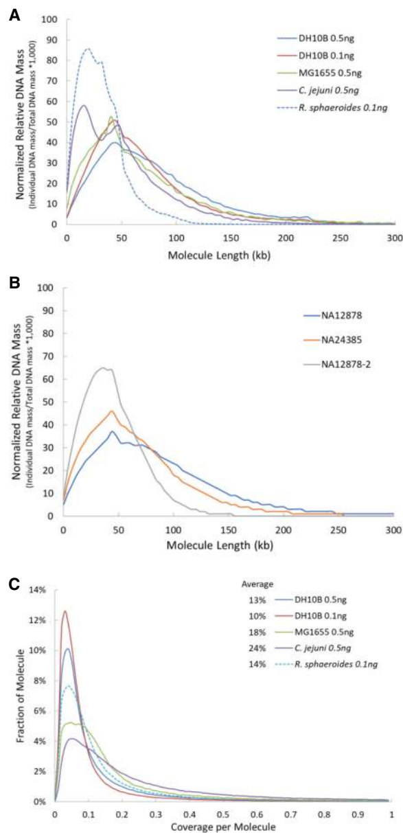
Figure 2. TELL-seq linked-read molecule analyses. (A) Calculated molecule length based on the TELL-seq sequencing data from microbial samples. To compare results from different microbial samples, the calculated DNA mass was normalized as follows: (Individual DNA mass at specified molecule length/Total DNA mass of the microbial sample) \times 1000. (B) Calculated molecule length based on the TELL-seq sequencing data from human cell line samples. To compare results from different samples, the calculated DNA mass was normalized as follows: (Individual DNA mass at specified molecule length/Total DNA mass of the cell line sample) \times 1000. (C) Distribution of linked-read sequencing coverage per molecule. Average sequencing coverage per molecule was 13%, 10%, 18%, 24%, and 14% for E. coli DH10B (0.5 ng genomic DNA input for library prep), E. coli DH10B (0.1 ng), E. coli K12 MG1655 (0.5 ng), C. jejuni (0.5 ng), and R. sphaeroides (0.1 ng), respectively.
