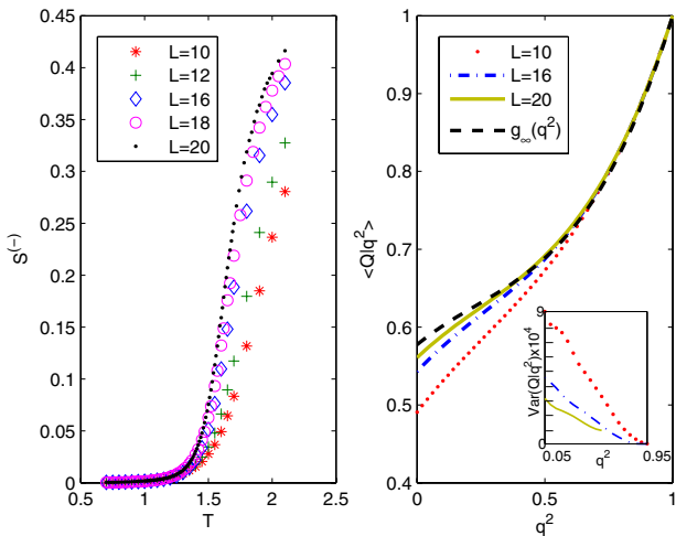
FIG. 4 (color online). Left-hand panel: The average value of S^{(-)} (defined in the text) as a function of T . Right-hand panel: Conditional expectation \langle Q|q^2 \rangle and conditional variance \text{Var}(Q|q^2) (inset) of the random variable Q given q^2 , where Q is the link overlap and q^2 is the square of the standard overlap, for different system sizes at temperature T = 0.7 .
