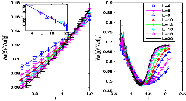
FIG. 3 (color online). Normalized variances of the two random variables \bar{x} = \bar{q}_{\text{med}} - \bar{q}_{\text{min}} (left) and \bar{y} = \bar{q}_{\text{max}} - \bar{q}_{\text{med}} (right) as a function of the temperature. The inset (at left) shows the L dependence of \text{Var}(\bar{x})/\text{Var}(|q|) at fixed temperature T = 0.7 on a log-log scale together with the best fit: \text{Var}(\bar{x})/\text{Var}(|q|) \sim aL^b , a = 0.12 , b = -0.23 .
