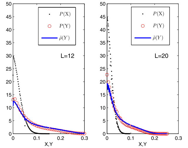
FIG. 2 (color online). Empirical distributions \mathcal{P}(X) and \mathcal{P}(Y) for X = Q_{\text{med}} - Q_{\text{min}} and Y = Q_{\text{max}} - Q_{\text{med}} for the two system sizes ( L = 12 and L = 20 ) at temperature T = 0.7 . \tilde{\rho}(Y) shows the distribution of Y computed from Eq. (5) using experimental data for \mathcal{P}(Q) and approximating the delta function with the histogram of X .
