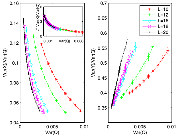
FIG. 1 (color online). Normalized variances of the two random variables X = Q_{\text{med}} - Q_{\text{min}} (left) and Y = Q_{\text{max}} - Q_{\text{med}} (right) as a function of \text{Var}(Q) . The inset (at left) shows the scaling law for \alpha = 1.18 , i.e., L^\alpha \text{Var}(X)/\text{Var}(Q) is L independent.
