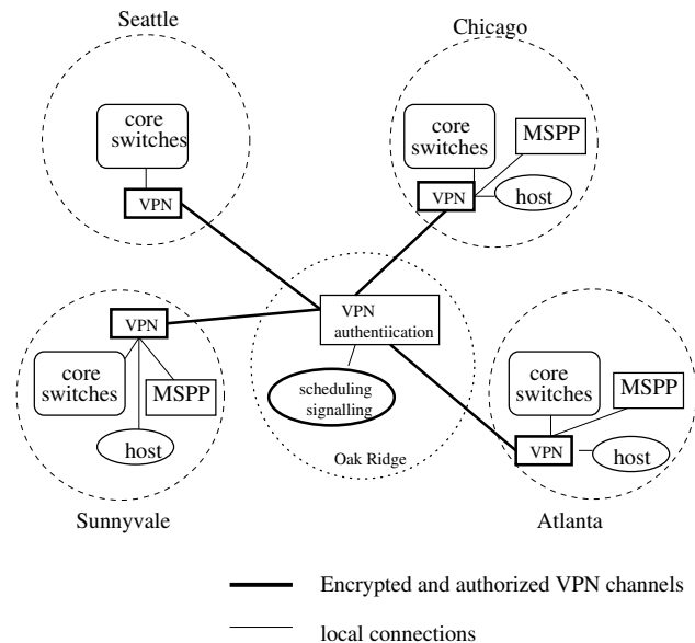
Fig. 5. Control-plane supported on VPN.
