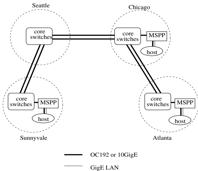
Fig. 2. Data Plane of UltraScienceNet consists of core switches and MSPPs.
