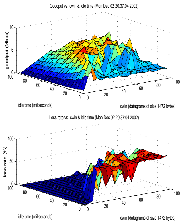
Fig. 9. Measurements for ORNL-LSU Internet Connection. Each point in horizontal plane represents a sending rate given by window size and idle time pair. Top plot corresponds to the goodput at the destination and the bottom plot corresponds to the loss rate.
