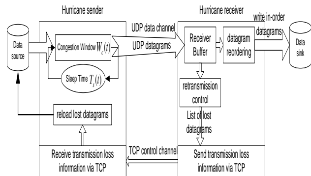
Fig. 11. Hurricane transport control structure.
