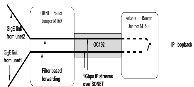
Fig. 7. Router configuration for implementing dedicated channel
