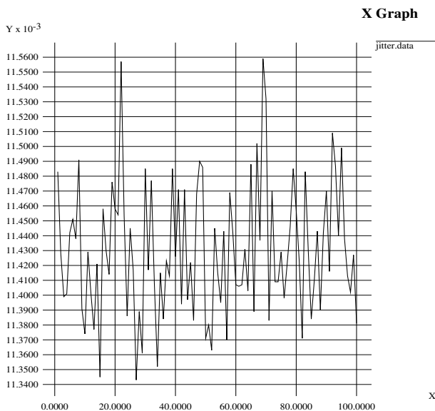
Fig. 10. Jitter levels over ORNL-Atlanta-ORNL dedicated channel
