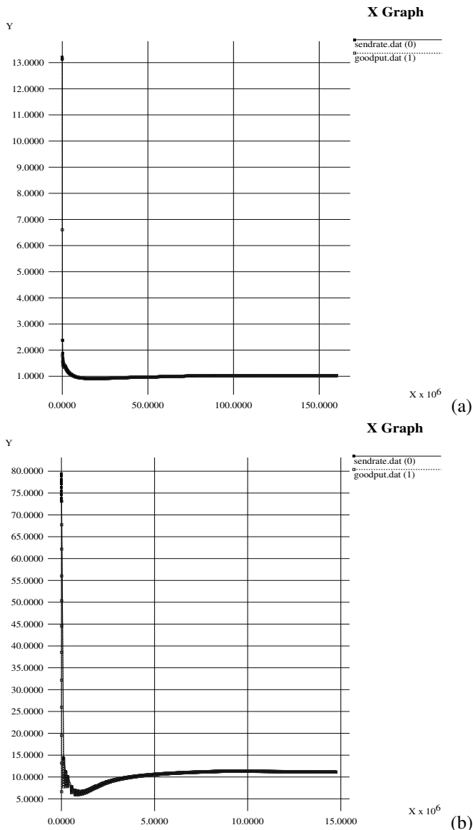
Fig. 13. Stabilization over the dedicated link: target goodput is 1.0 and 10.0 Mbps in (a) and (b) respectively; a = 0.8 , \alpha = 0.8 , adjustment is made on sleep time.
