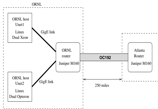
Fig. 6. ORNL-Atlanta-ORNL dedicated 1 Gbps IP connection.
