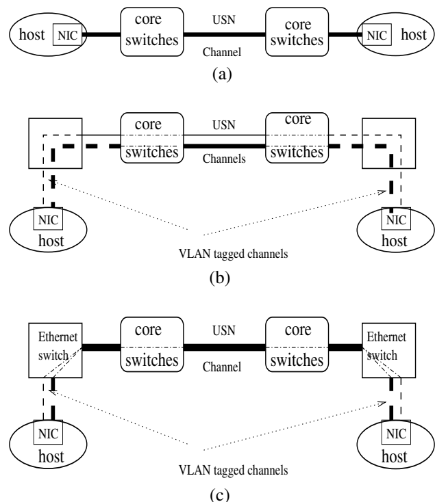
Fig. 3. Connecting hosts to USN channels: (a) NICs directly connected to core switches, (b) VLAN tagging to utilize multiple USN channels, and (c) VLAN tagging to share single USN channels.
