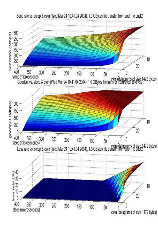
Fig. 8. Measurements for ORNL-Atlanta-ORNL dedicated 1Gbps IP channel. Each point in horizontal plane represents sending rate given by window size and idle time pair. Top plot corresponds to sending rate, middle plot corresponds to the goodput at the destination and the bottom plot corresponds to the loss rate.
