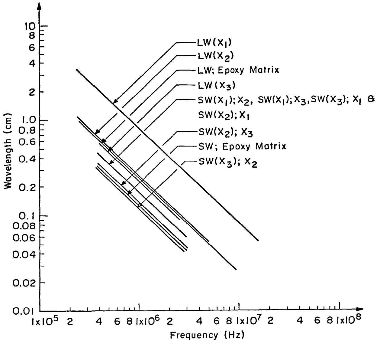
Fig. 14 Wavelengths versus frequency for longitudinal and shear waves in various specimens for the indicated directions.
