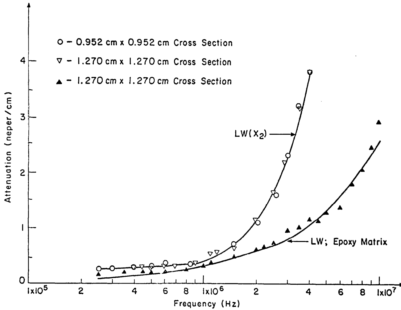
Fig. 9 Attenuation of longitudinal wave for the indicated specimens and directions.
