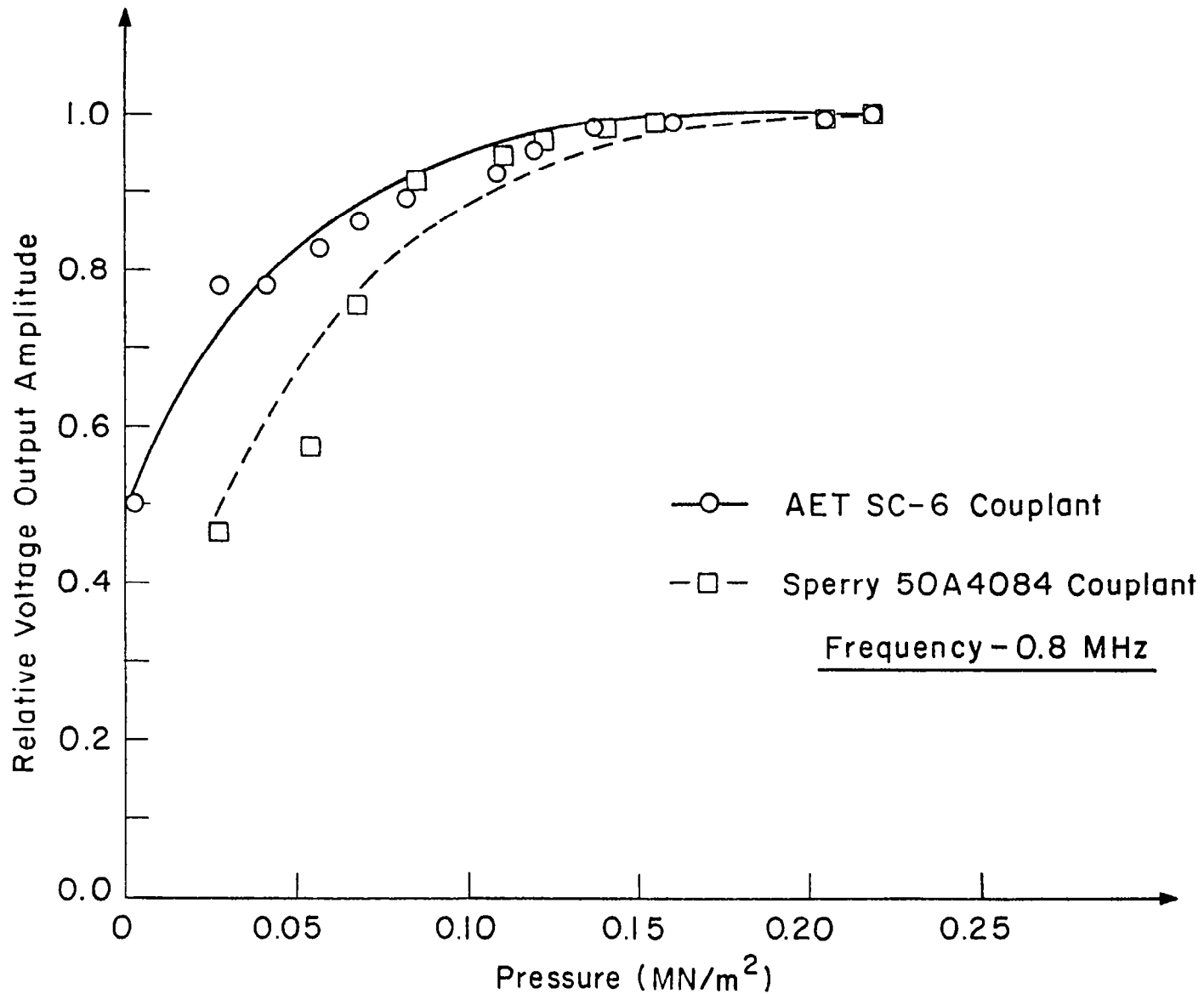
Fig. 4 Variation of relative output amplitude versus transducer-specimen interface pressure.
