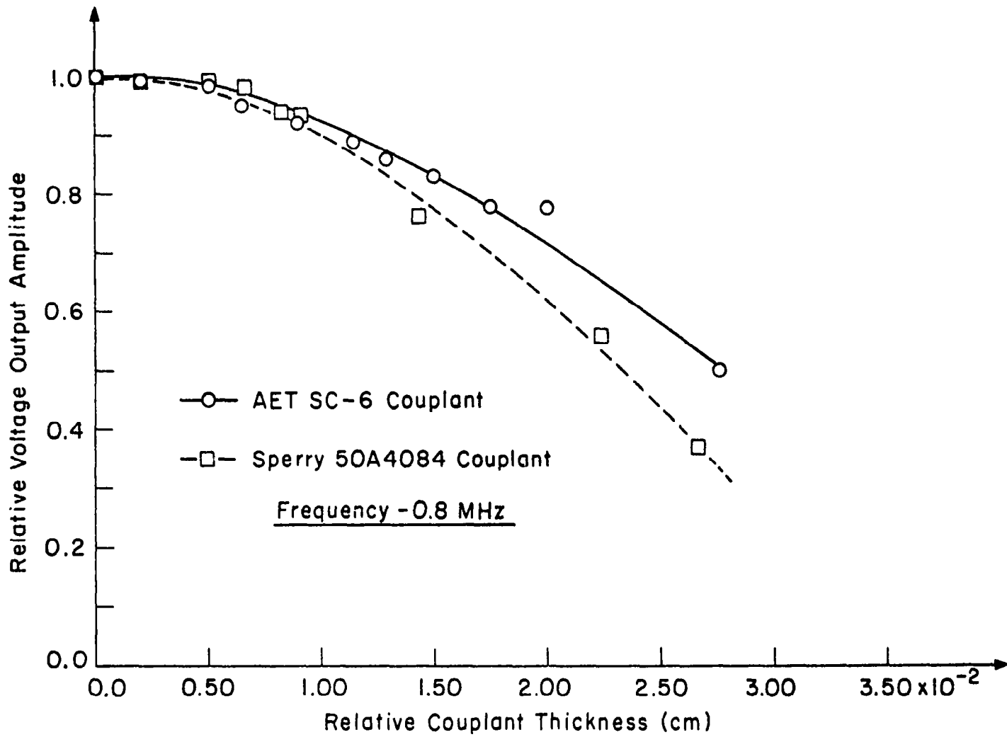
Fig. 5 Variation of relative output amplitude versus relative couplant thickness ( \delta - \delta_{\min} ).
