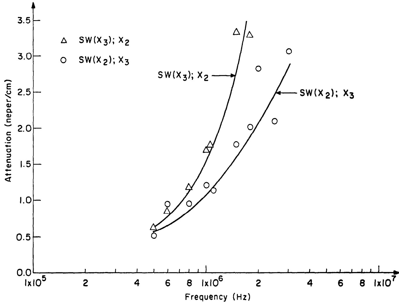
Fig. 13 Attenuation of shear wave in the indicated directions and specimens. (Specimens had 1.270 cm x 1.270 cm Cross Section.)
