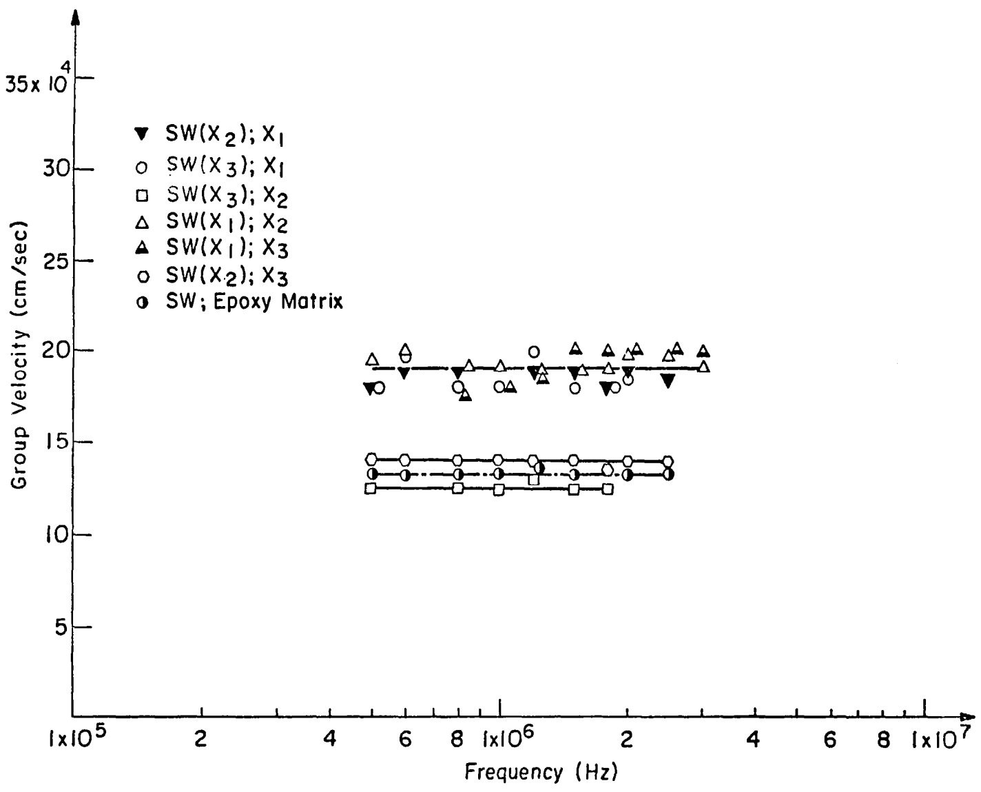
Fig. 11 Shear wave group velocities versus frequency for the indicated specimens and directions. (Specimens had 1.270 cm x 1.270 cm Cross Section.)
