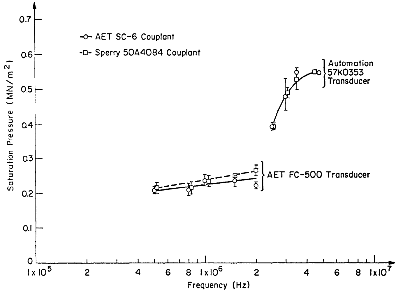
Fig. 6 Variation of saturation pressure versus signal frequency for two longitudinal transducers.
