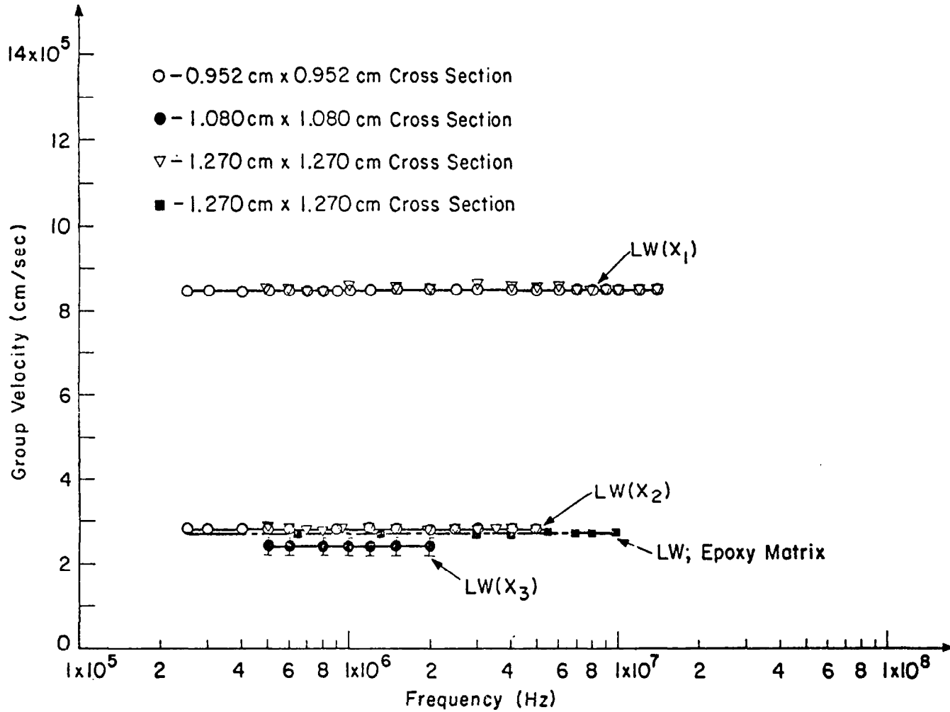
Fig. 7 Longitudinal group velocities versus frequency for the indicated specimens and directions.
