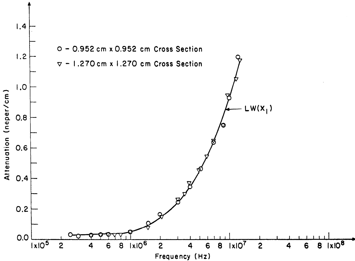
Fig. 8 Attenuation of longitudinal wave versus frequency for 0° specimen.
