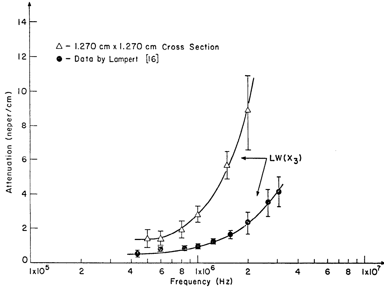
Fig. 10 Attenuation of longitudinal wave perpendicular to the laminate versus frequency for 90° specimen. (Mean values are plotted with brackets indicating the standard deviation about the mean.)
