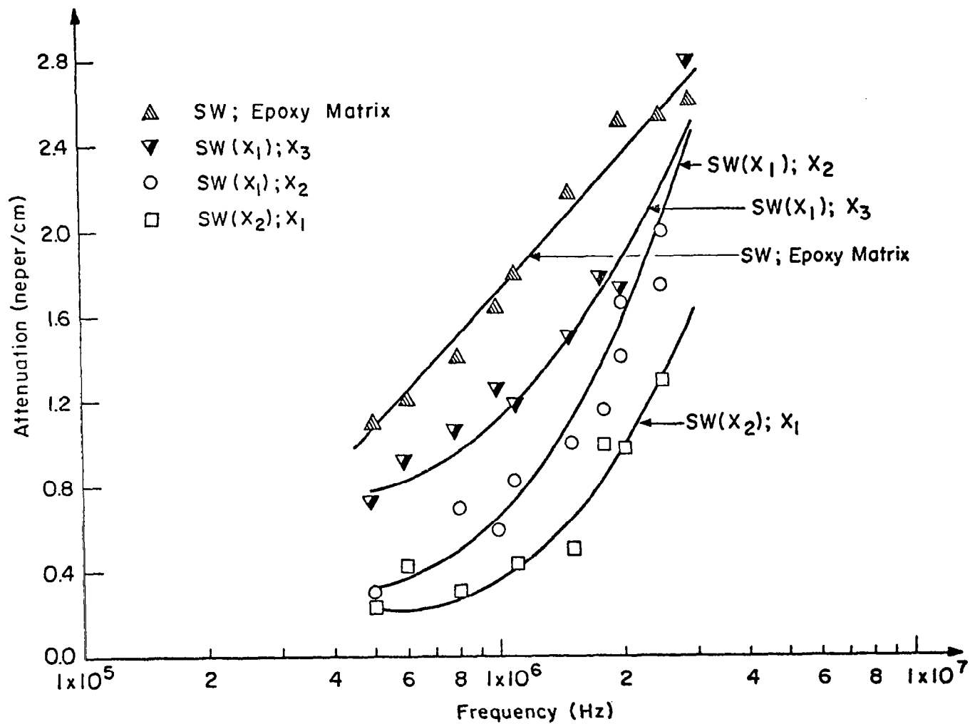
Fig. 12 Attenuation of shear wave in the indicated directions and specimens. (Specimens had 1.270 cm x 1.270 cm Cross Section.)
